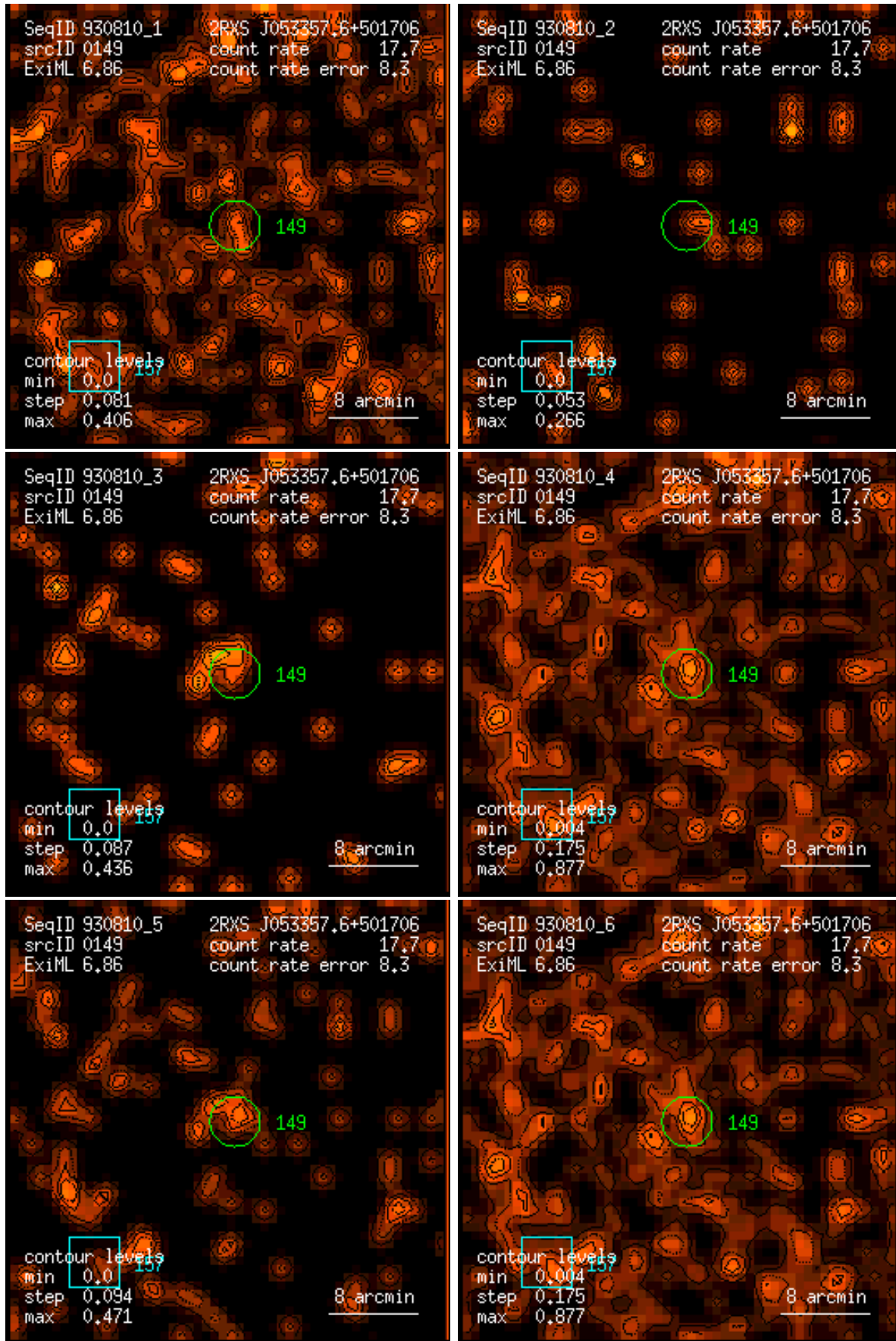
Figure 149: RASS 930810: detection 0149: band rate images, Gaussian filter: (1) PSPC channels 11 – 41, (2) 52 – 90, (3) 91 – 201, (4) 11 – 235, (5) 52 – 201, (6) 11 – 201. Broad band rates in counts/ks. Band rate contour levels in counts/ks/arcmin 2 .
