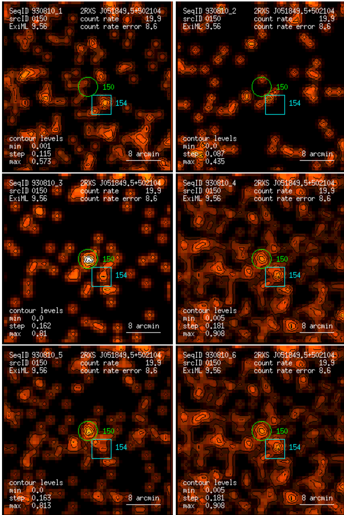
Figure 150: RASS 930810: detection 0150: band rate images, Gaussian filter: (1) PSPC channels 11 – 41, (2) 52 – 90, (3) 91 – 201, (4) 11 – 235, (5) 52 – 201, (6) 11 – 201. Broad band rates in counts/ks. Band rate contour levels in counts/ks/arcmin 2 .
