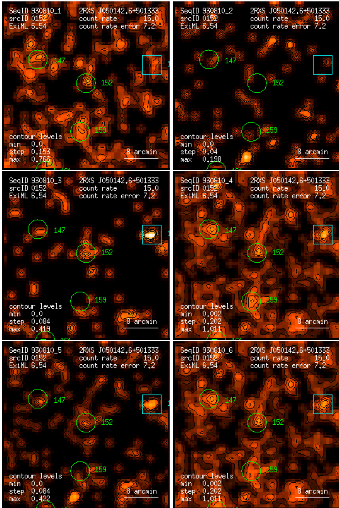
Figure 152: RASS 930810: detection 0152: band rate images, Gaussian filter: (1) PSPC channels 11 – 41, (2) 52 – 90, (3) 91 – 201, (4) 11 – 235, (5) 52 – 201, (6) 11 – 201. Broad band rates in counts/ks. Band rate contour levels in counts/ks/arcmin 2 .
