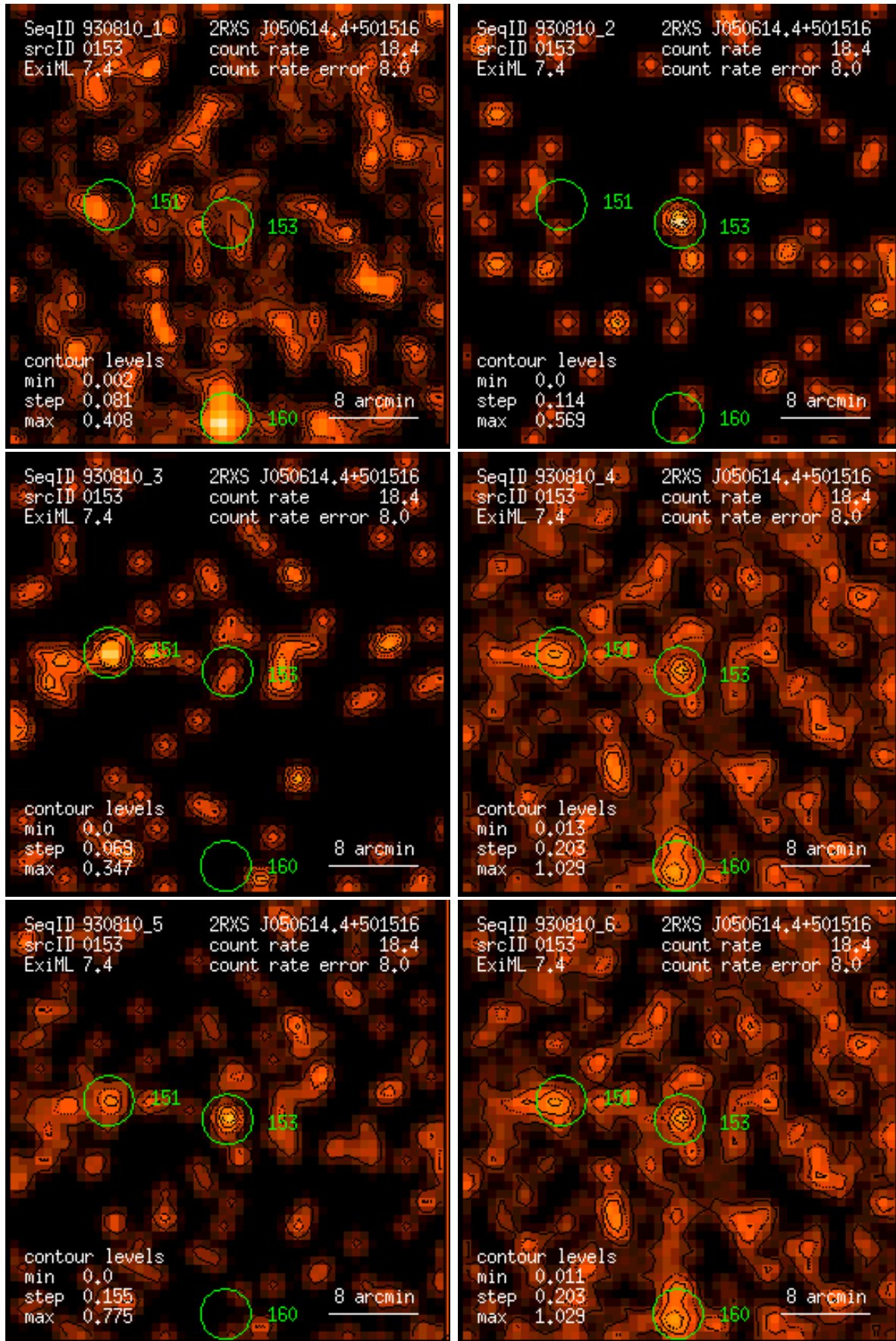
Figure 153: RASS 930810: detection 0153: band rate images, Gaussian filter: (1) PSPC channels 11 – 41, (2) 52 – 90, (3) 91 – 201, (4) 11 – 235, (5) 52 – 201, (6) 11 – 201. Broad band rates in counts/ks. Band rate contour levels in counts/ks/arcmin 2 .
