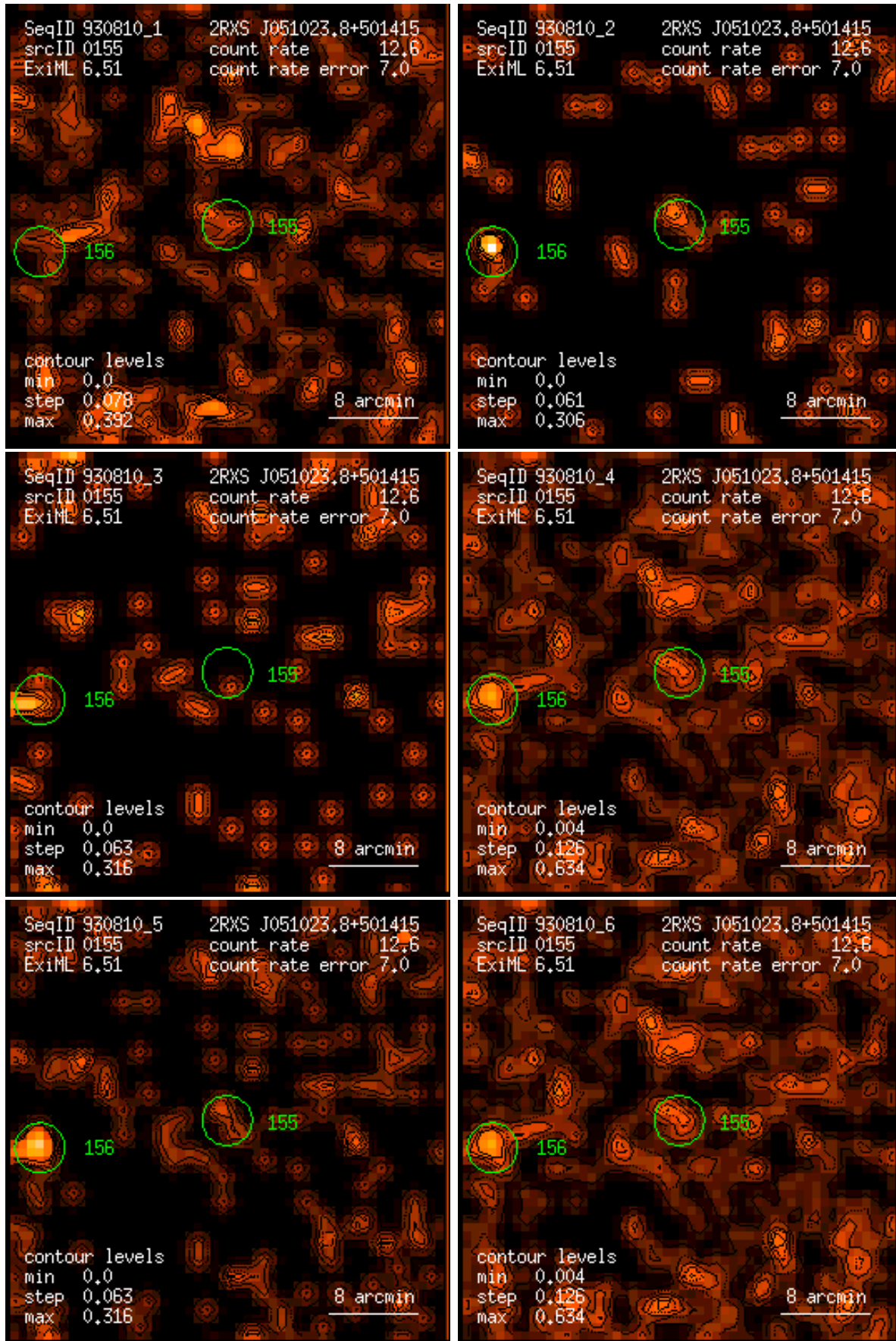
Figure 155: RASS 930810: detection 0155: band rate images, Gaussian filter: (1) PSPC channels 11 – 41, (2) 52 – 90, (3) 91 – 201, (4) 11 – 235, (5) 52 – 201, (6) 11 – 201. Broad band rates in counts/ks. Band rate contour levels in counts/ks/arcmin 2 .
