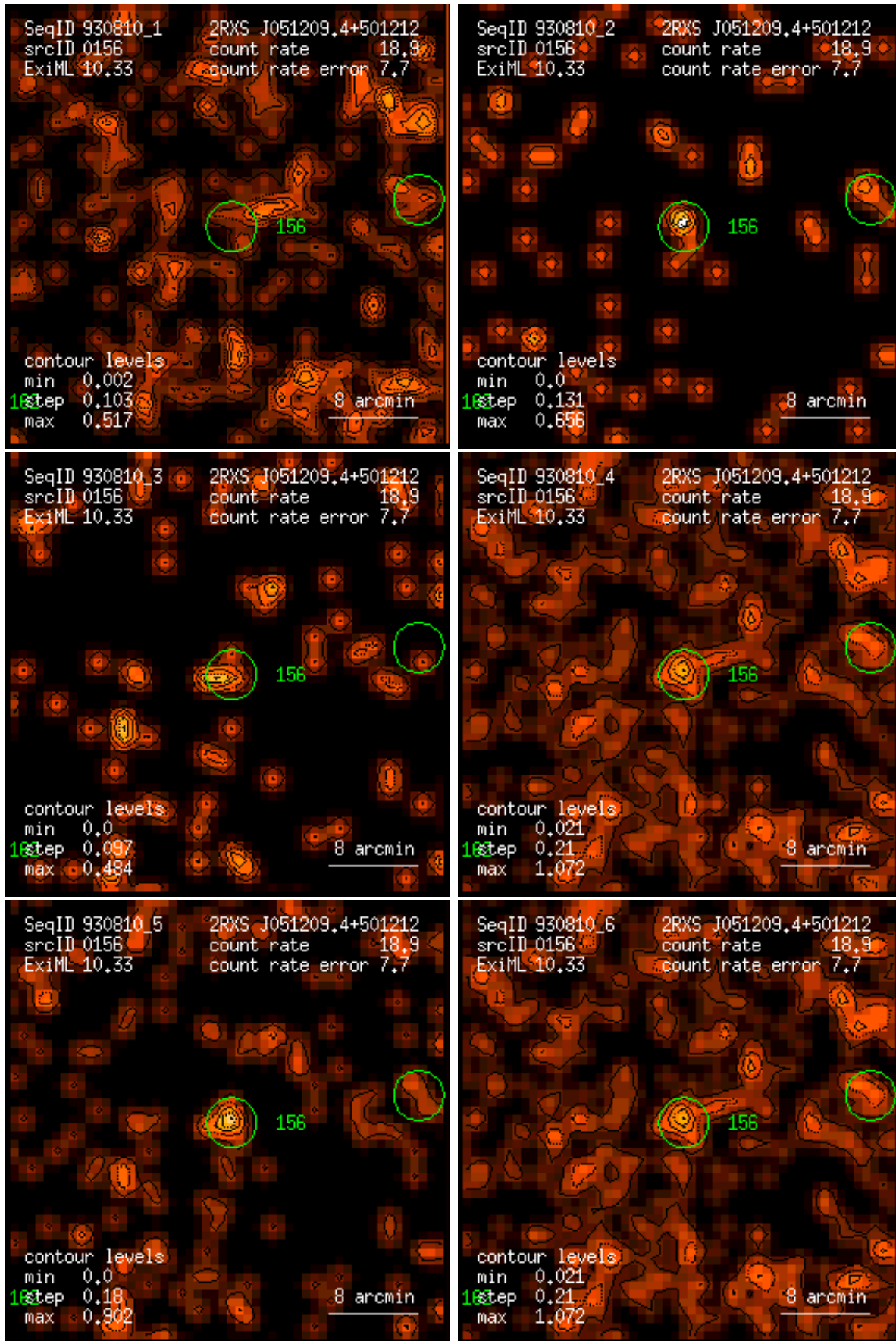
Figure 156: RASS 930810: detection 0156: band rate images, Gaussian filter: (1) PSPC channels 11 – 41, (2) 52 – 90, (3) 91 – 201, (4) 11 – 235, (5) 52 – 201, (6) 11 – 201. Broad band rates in counts/ks. Band rate contour levels in counts/ks/arcmin 2 .
