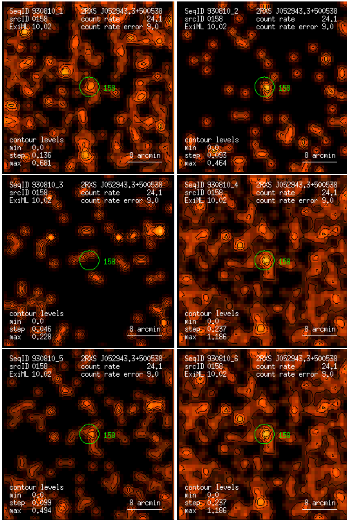
Figure 158: RASS 930810: detection 0158: band rate images, Gaussian filter: (1) PSPC channels 11 – 41, (2) 52 – 90, (3) 91 – 201, (4) 11 – 235, (5) 52 – 201, (6) 11 – 201. Broad band rates in counts/ks. Band rate contour levels in counts/ks/arcmin 2 .
