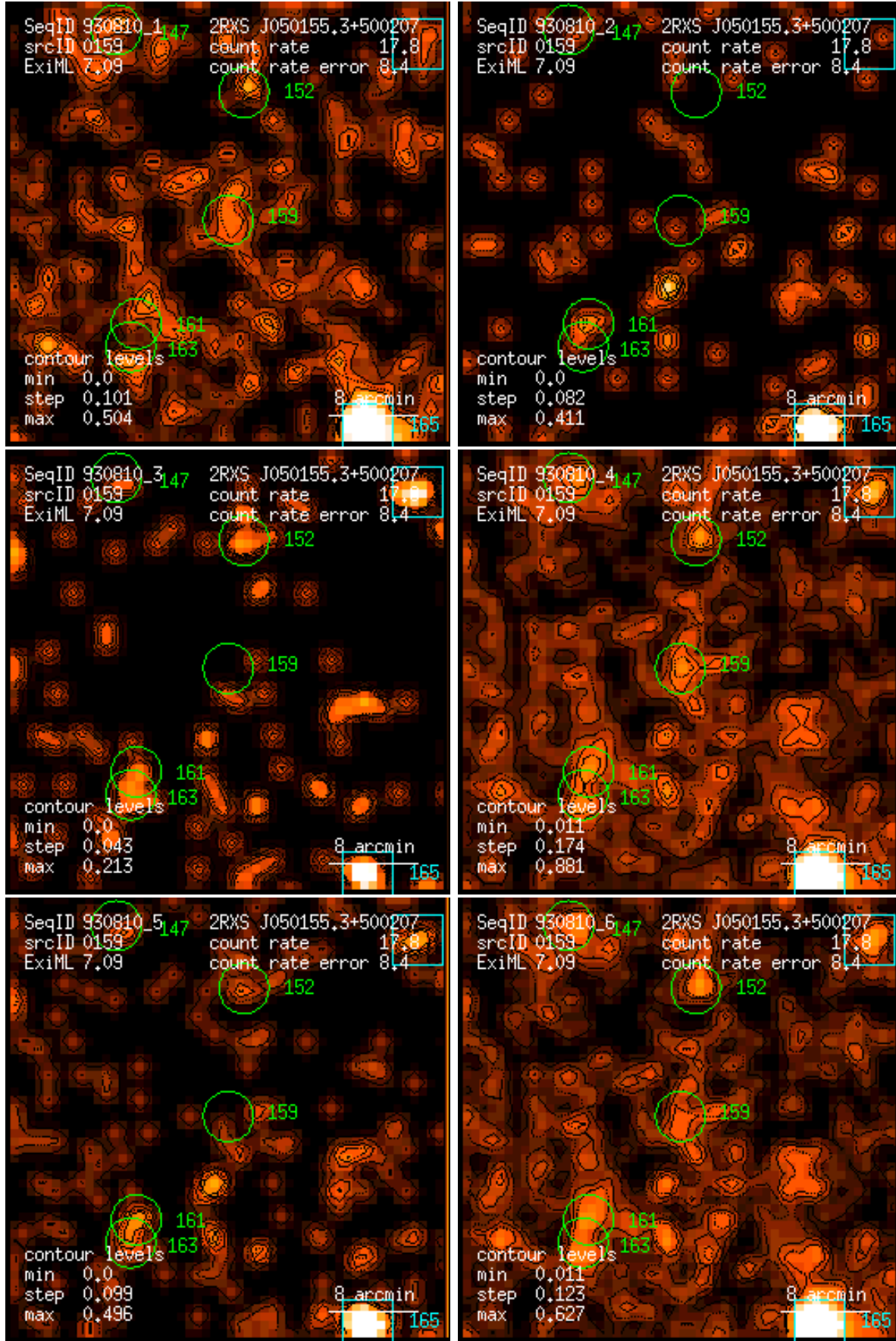
Figure 159: RASS 930810: detection 0159: band rate images, Gaussian filter: (1) PSPC channels 11 – 41, (2) 52 – 90, (3) 91 – 201, (4) 11 – 235, (5) 52 – 201, (6) 11 – 201. Broad band rates in counts/ks. Band rate contour levels in counts/ks/arcmin 2 .
