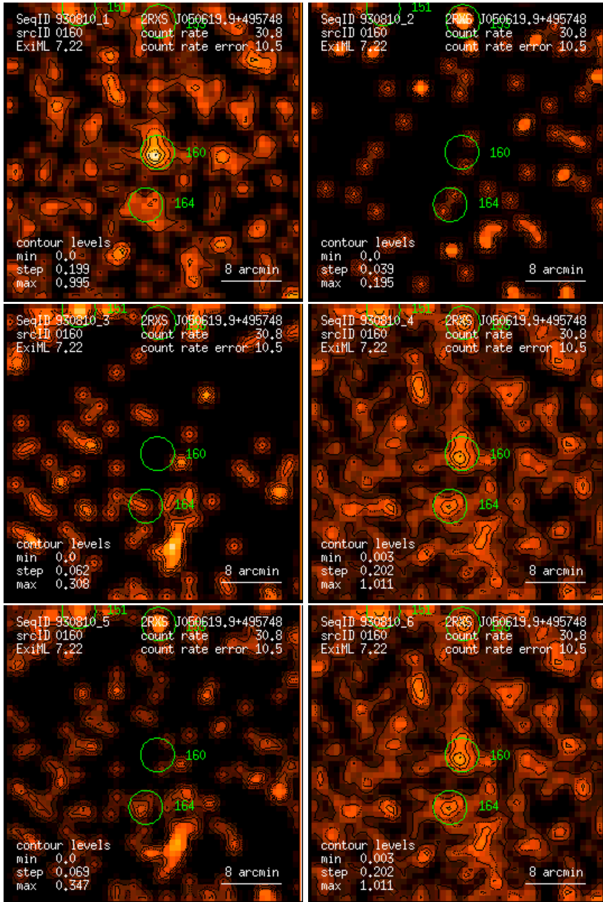
Figure 160: RASS 930810: detection 0160: band rate images, Gaussian filter: (1) PSPC channels 11 – 41, (2) 52 – 90, (3) 91 – 201, (4) 11 – 235, (5) 52 – 201, (6) 11 – 201. Broad band rates in counts/ks. Band rate contour levels in counts/ks/arcmin 2 .
