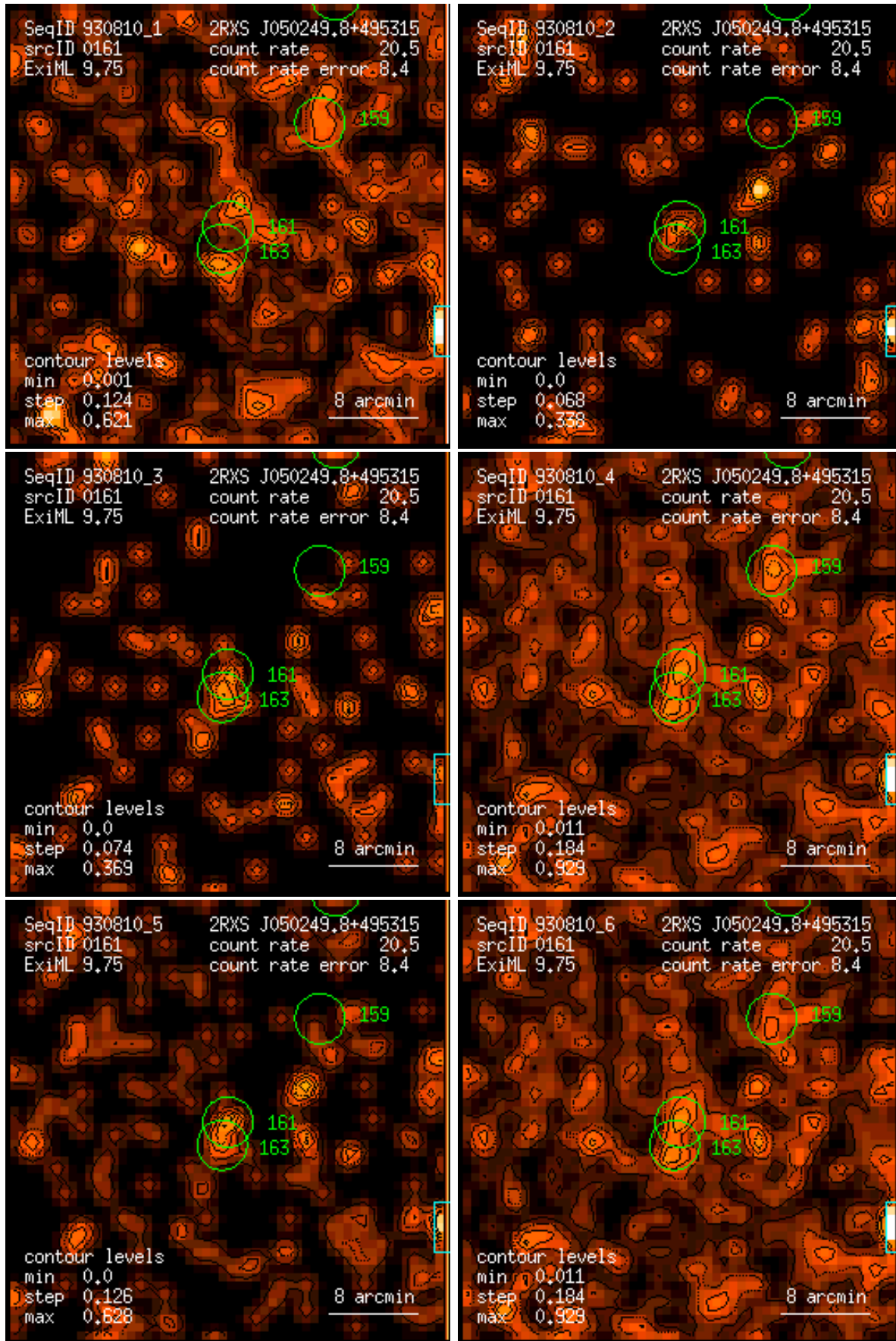
Figure 161: RASS 930810: detection 0161: band rate images, Gaussian filter: (1) PSPC channels 11 – 41, (2) 52 – 90, (3) 91 – 201, (4) 11 – 235, (5) 52 – 201, (6) 11 – 201. Broad band rates in counts/ks. Band rate contour levels in counts/ks/arcmin 2 .
