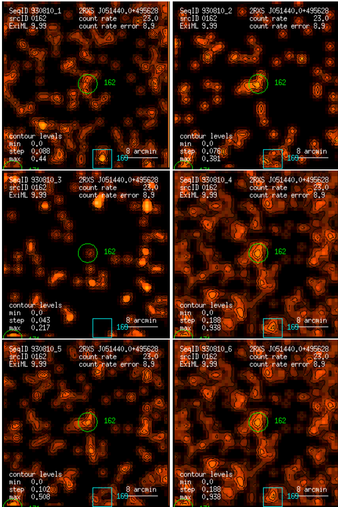
Figure 162: RASS 930810: detection 0162: band rate images, Gaussian filter: (1) PSPC channels 11 – 41, (2) 52 – 90, (3) 91 – 201, (4) 11 – 235, (5) 52 – 201, (6) 11 – 201. Broad band rates in counts/ks. Band rate contour levels in counts/ks/arcmin 2 .
