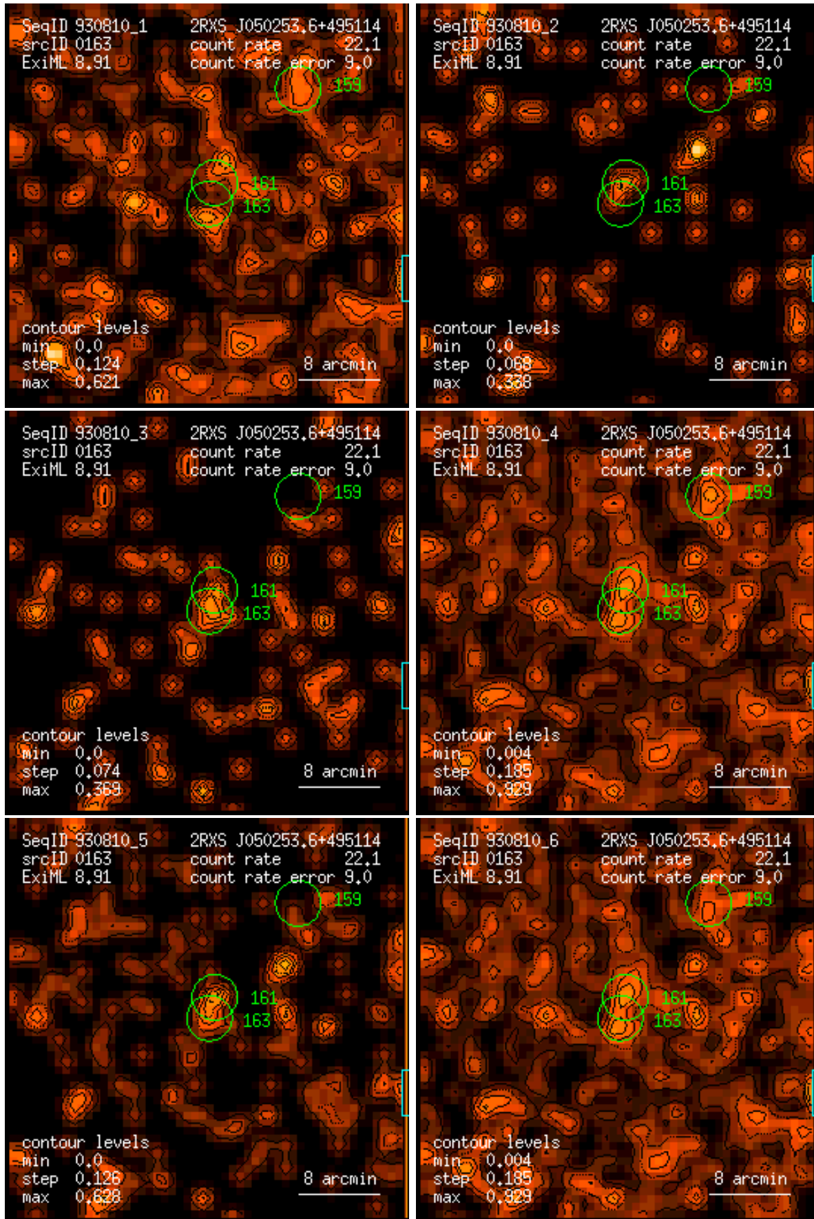
Figure 163: RASS 930810: detection 0163: band rate images, Gaussian filter: (1) PSPC channels 11 – 41, (2) 52 – 90, (3) 91 – 201, (4) 11 – 235, (5) 52 – 201, (6) 11 – 201. Broad band rates in counts/ks. Band rate contour levels in counts/ks/arcmin 2 .
