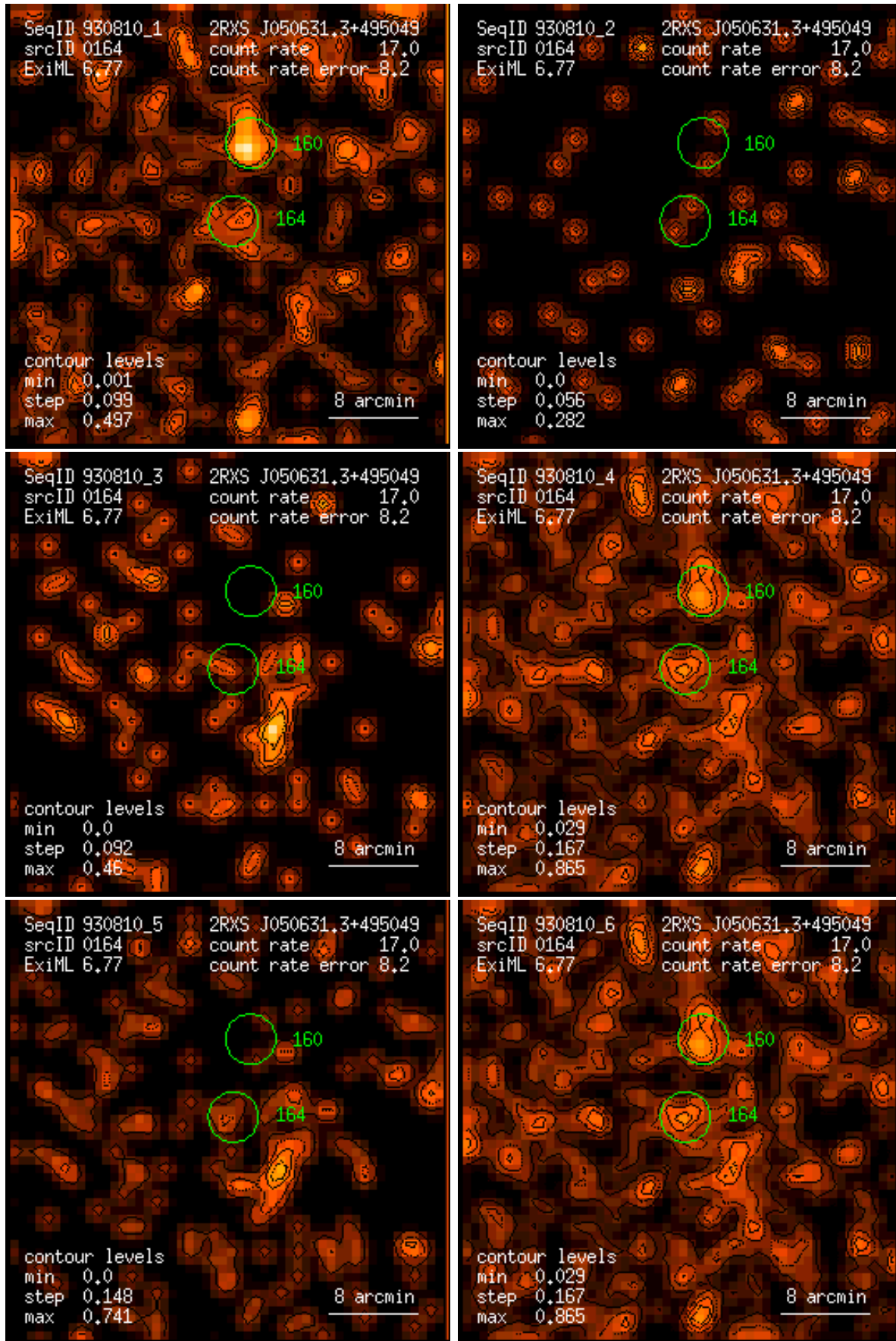
Figure 164: RASS 930810: detection 0164: band rate images, Gaussian filter: (1) PSPC channels 11 – 41, (2) 52 – 90, (3) 91 – 201, (4) 11 – 235, (5) 52 – 201, (6) 11 – 201. Broad band rates in counts/ks. Band rate contour levels in counts/ks/arcmin 2 .
