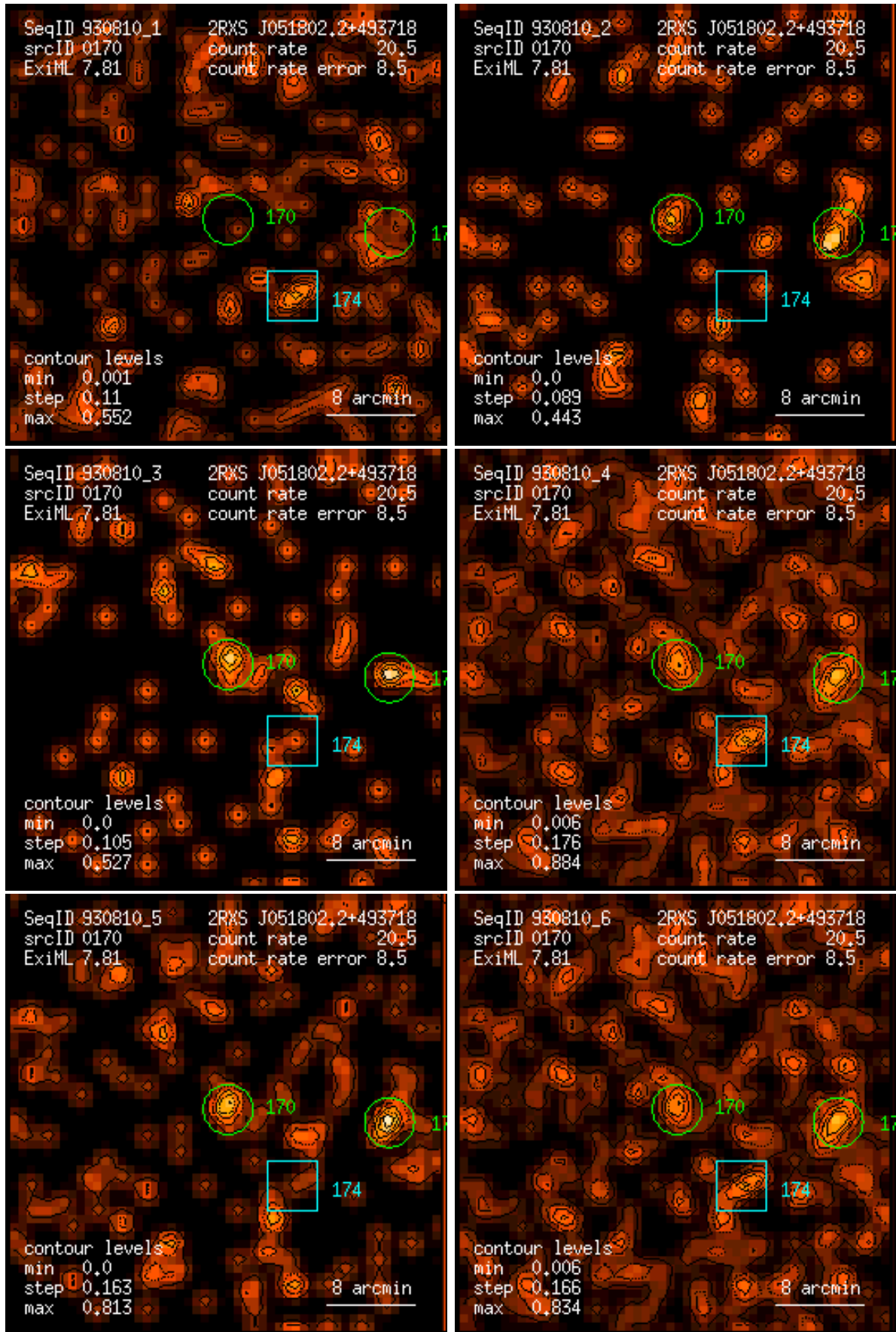
Figure 170: RASS 930810: detection 0170: band rate images, Gaussian filter: (1) PSPC channels 11 – 41, (2) 52 – 90, (3) 91 – 201, (4) 11 – 235, (5) 52 – 201, (6) 11 – 201. Broad band rates in counts/ks. Band rate contour levels in counts/ks/arcmin 2 .
