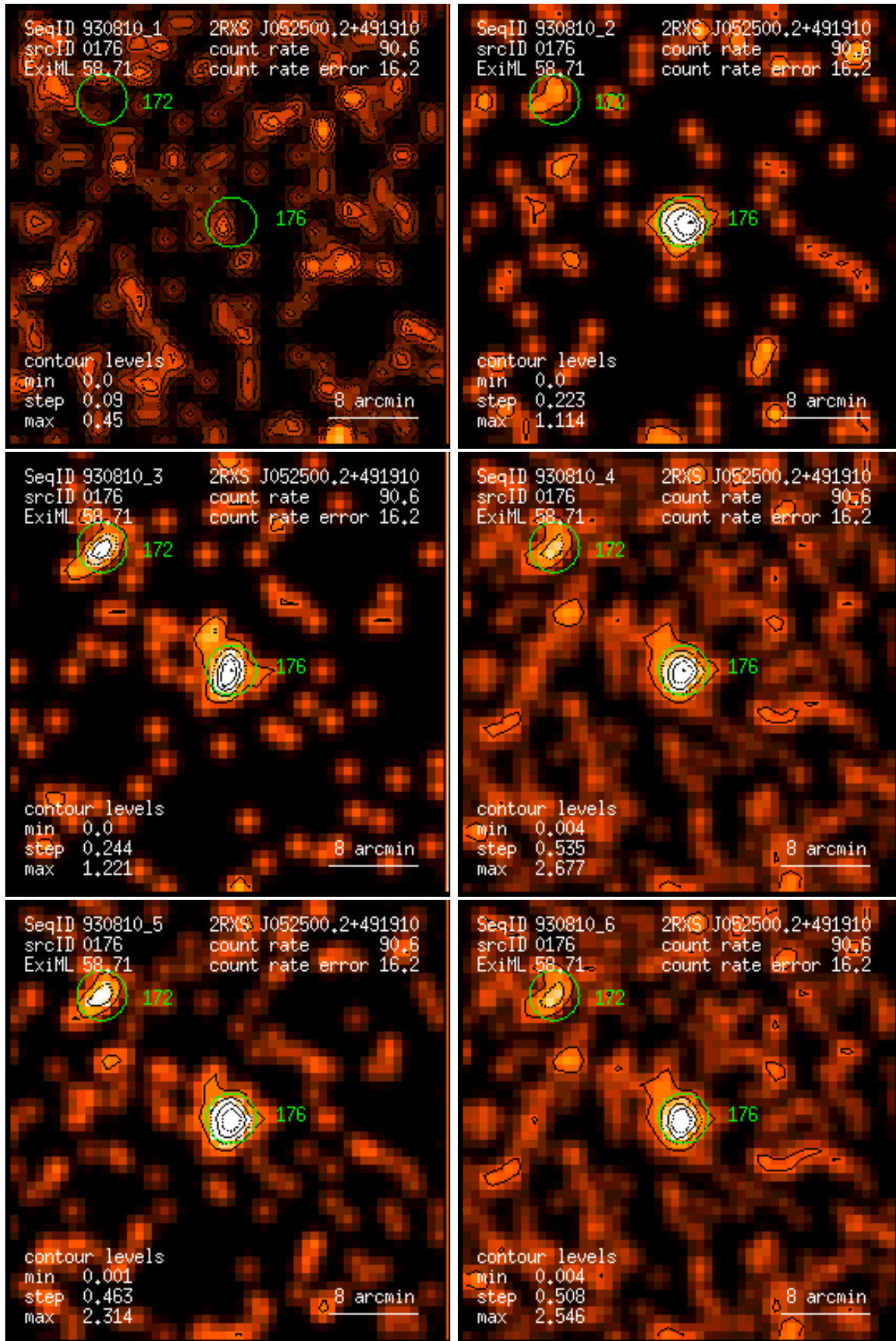
Figure 176: RASS 930810: detection 0176: band rate images, Gaussian filter: (1) PSPC channels 11 – 41, (2) 52 – 90, (3) 91 – 201, (4) 11 – 235, (5) 52 – 201, (6) 11 – 201. Broad band rates in counts/ks. Band rate contour levels in counts/ks/arcmin 2 .
