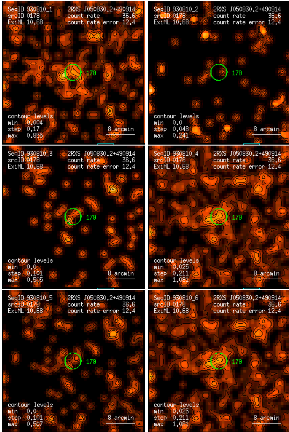
Figure 178: RASS 930810: detection 0178: band rate images, Gaussian filter: (1) PSPC channels 11 – 41, (2) 52 – 90, (3) 91 – 201, (4) 11 – 235, (5) 52 – 201, (6) 11 – 201. Broad band rates in counts/ks. Band rate contour levels in counts/ks/arcmin 2 .
