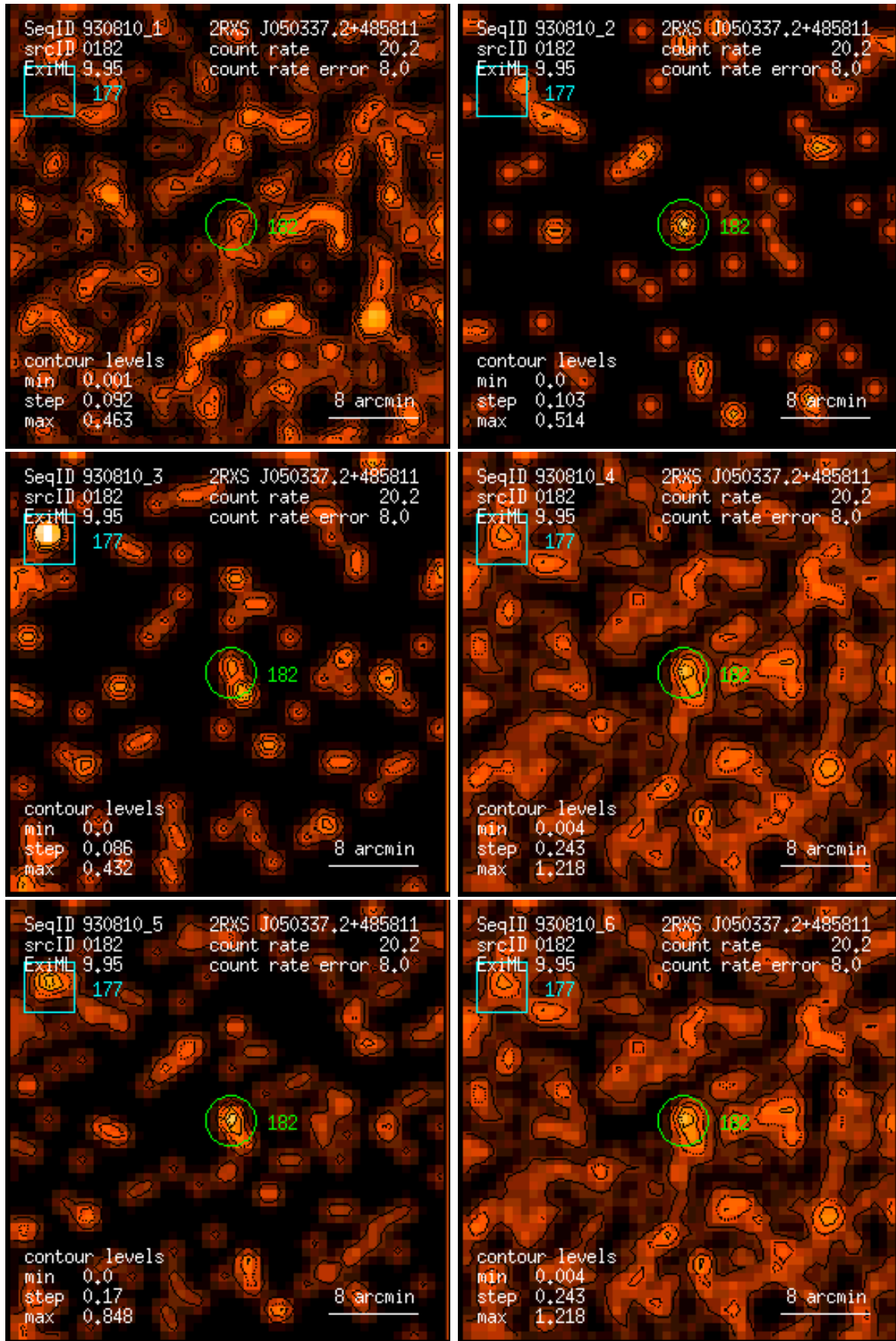
Figure 182: RASS 930810: detection 0182: band rate images, Gaussian filter: (1) PSPC channels 11 – 41, (2) 52 – 90, (3) 91 – 201, (4) 11 – 235, (5) 52 – 201, (6) 11 – 201. Broad band rates in counts/ks. Band rate contour levels in counts/ks/arcmin 2 .
