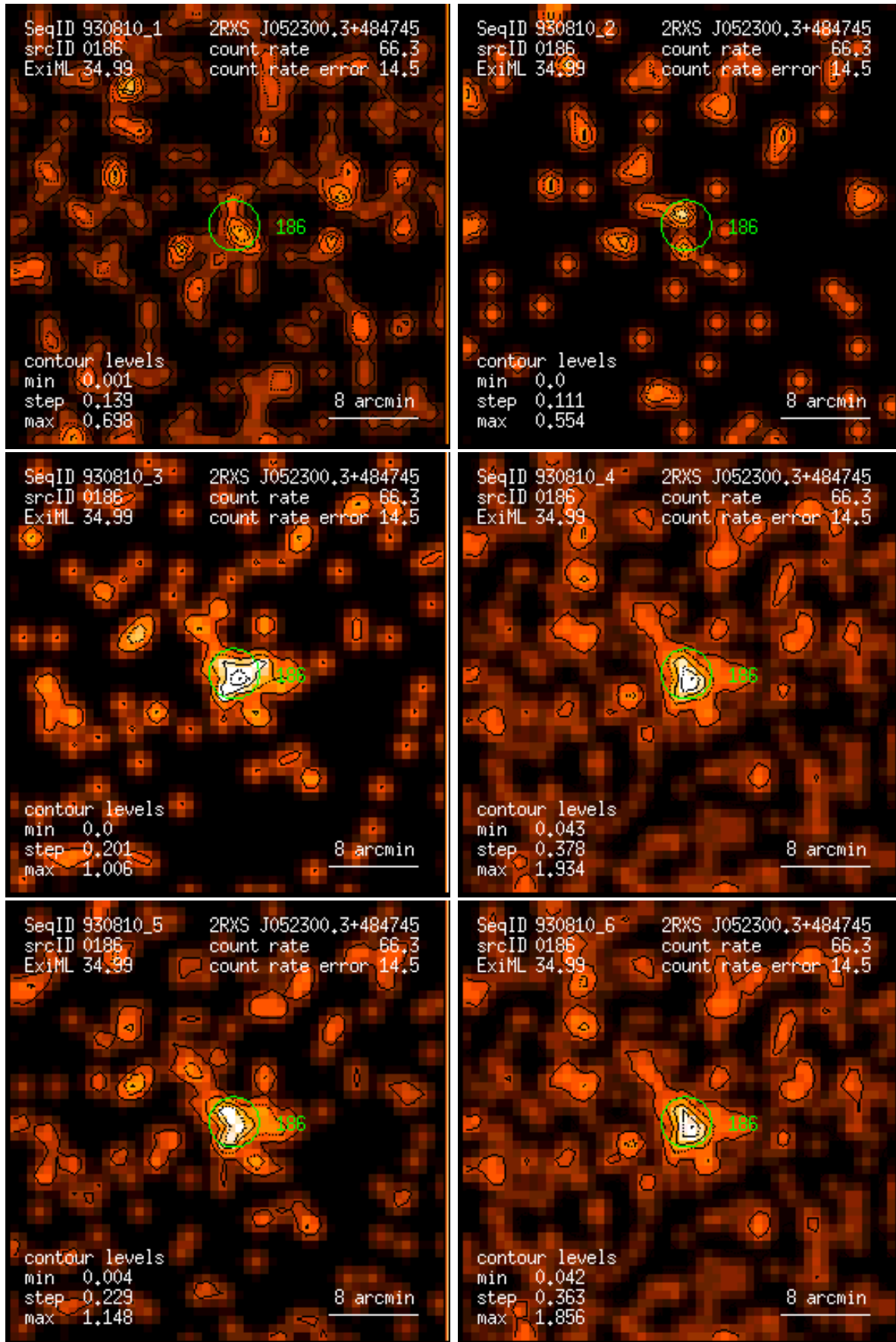
Figure 186: RASS 930810: detection 0186: band rate images, Gaussian filter: (1) PSPC channels 11 – 41, (2) 52 – 90, (3) 91 – 201, (4) 11 – 235, (5) 52 – 201, (6) 11 – 201. Broad band rates in counts/ks. Band rate contour levels in counts/ks/arcmin 2 .
