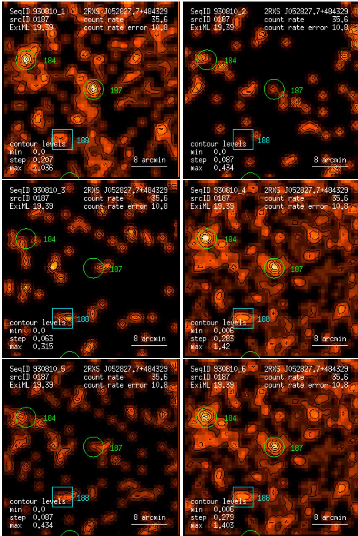
Figure 187: RASS 930810: detection 0187: band rate images, Gaussian filter: (1) PSPC channels 11 – 41, (2) 52 – 90, (3) 91 – 201, (4) 11 – 235, (5) 52 – 201, (6) 11 – 201. Broad band rates in counts/ks. Band rate contour levels in counts/ks/arcmin 2 .
