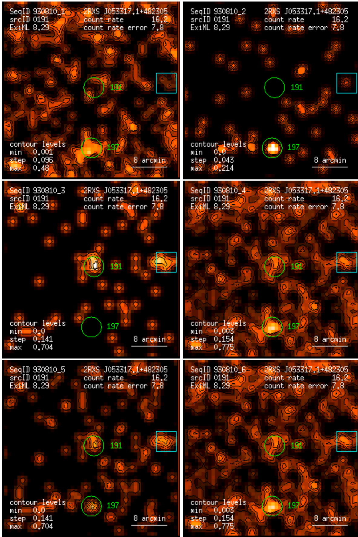
Figure 191: RASS 930810: detection 0191: band rate images, Gaussian filter: (1) PSPC channels 11 – 41, (2) 52 – 90, (3) 91 – 201, (4) 11 – 235, (5) 52 – 201, (6) 11 – 201. Broad band rates in counts/ks. Band rate contour levels in counts/ks/arcmin 2 .
