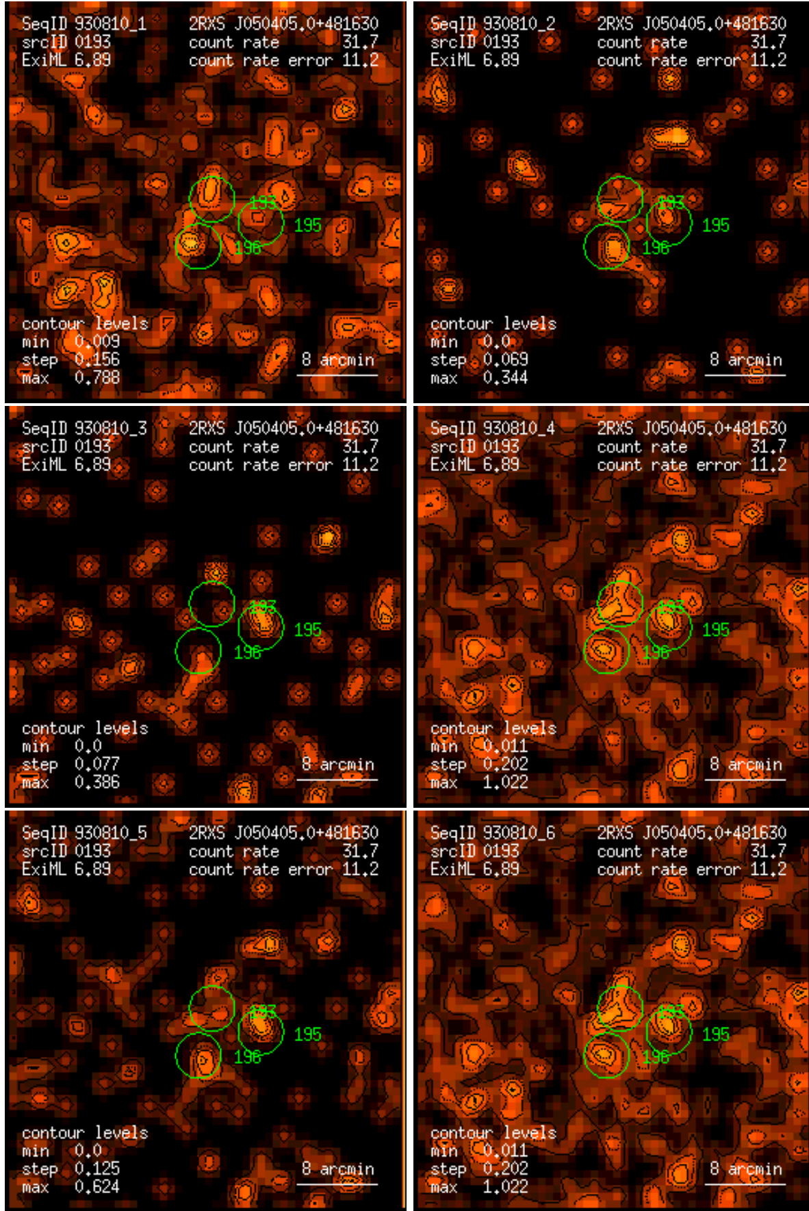
Figure 193: RASS 930810: detection 0193: band rate images, Gaussian filter: (1) PSPC channels 11 – 41, (2) 52 – 90, (3) 91 – 201, (4) 11 – 235, (5) 52 – 201, (6) 11 – 201. Broad band rates in counts/ks. Band rate contour levels in counts/ks/arcmin 2 .
