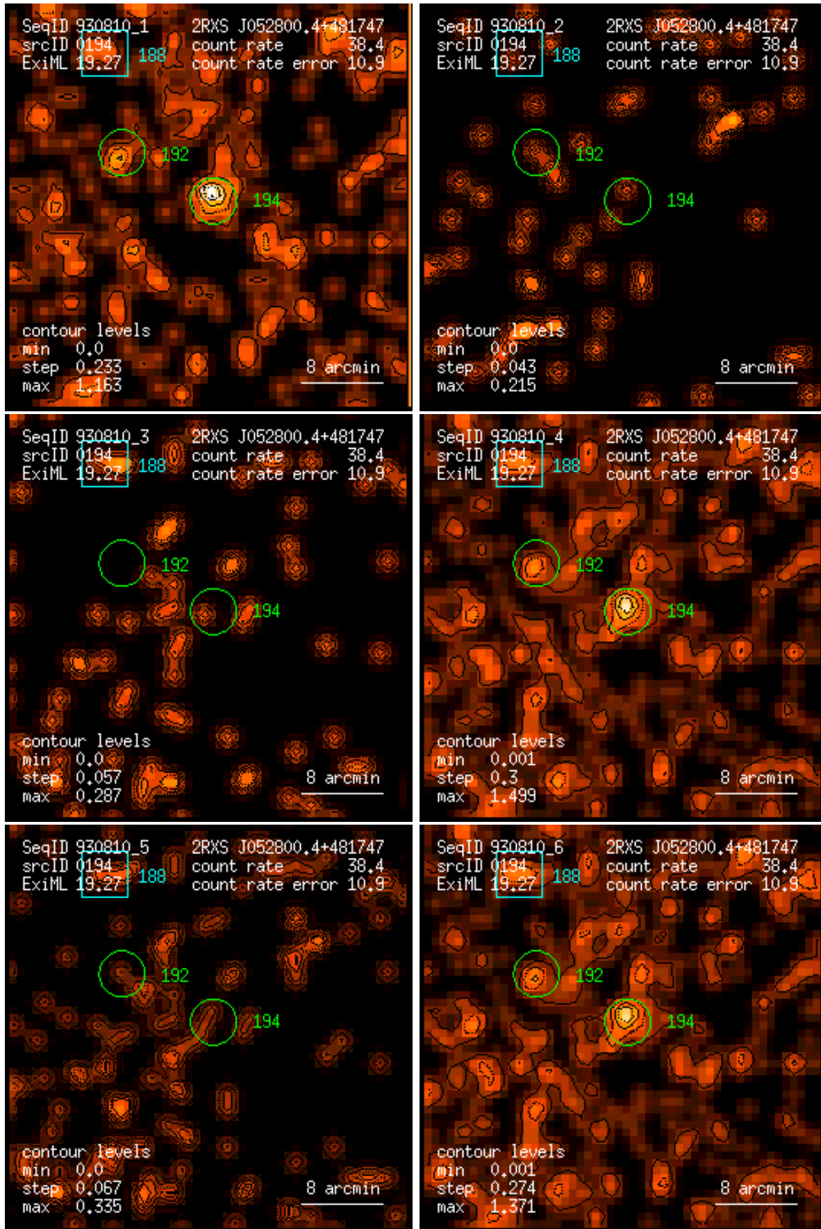
Figure 194: RASS 930810: detection 0194: band rate images, Gaussian filter: (1) PSPC channels 11 – 41, (2) 52 – 90, (3) 91 – 201, (4) 11 – 235, (5) 52 – 201, (6) 11 – 201. Broad band rates in counts/ks. Band rate contour levels in counts/ks/arcmin 2 .
