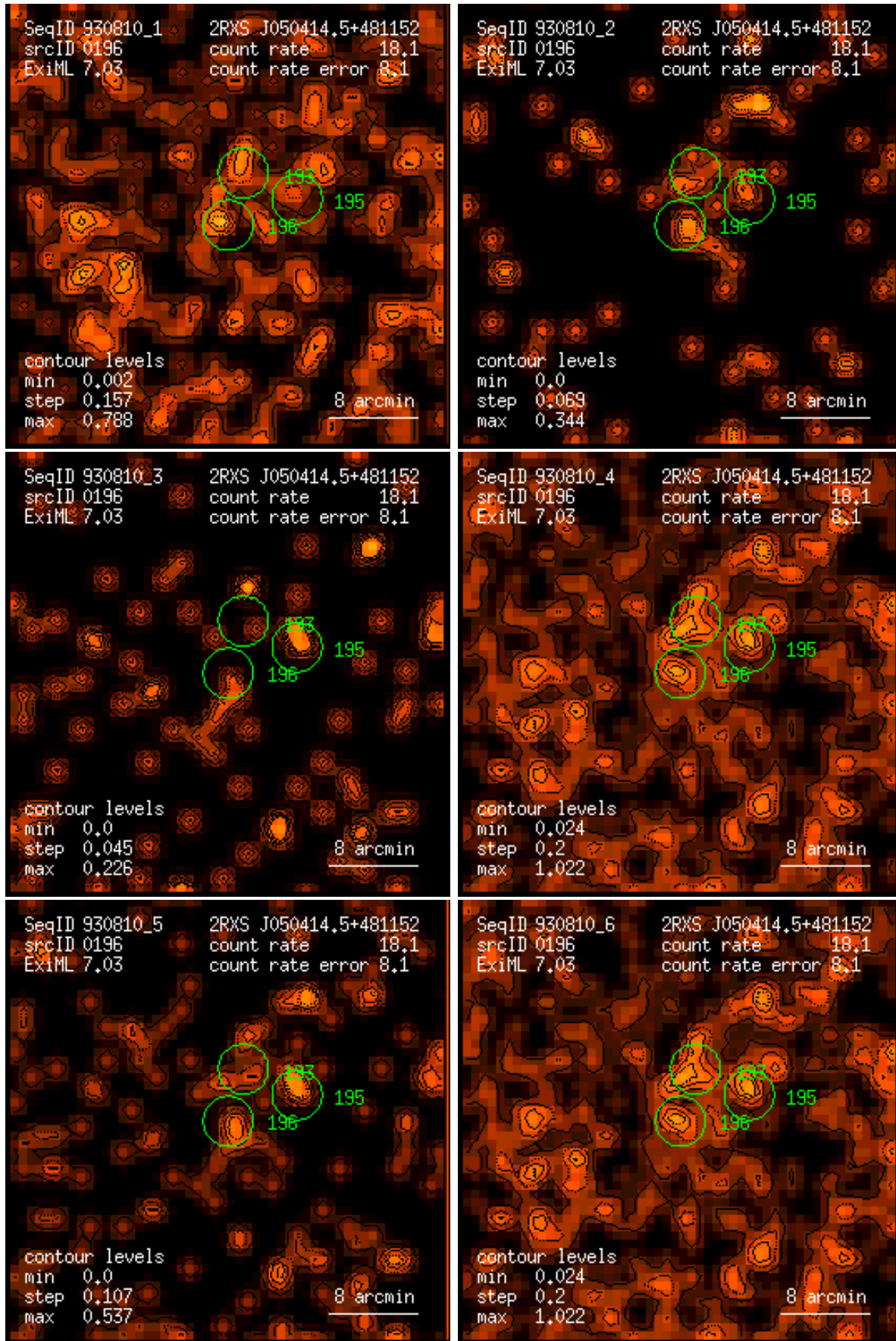
Figure 196: RASS 930810: detection 0196: band rate images, Gaussian filter: (1) PSPC channels 11 – 41, (2) 52 – 90, (3) 91 – 201, (4) 11 – 235, (5) 52 – 201, (6) 11 – 201. Broad band rates in counts/ks. Band rate contour levels in counts/ks/arcmin 2 .
