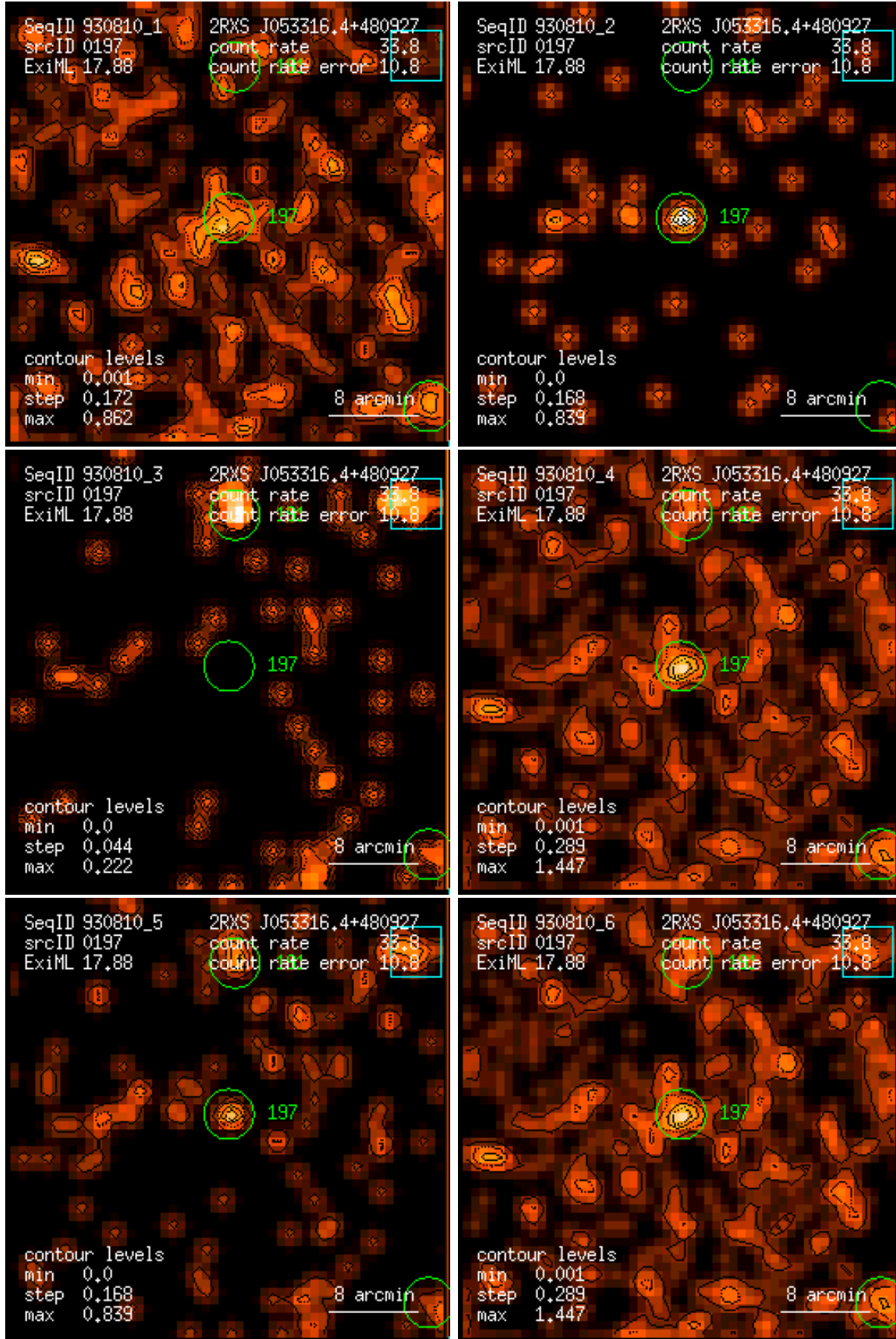
Figure 197: RASS 930810: detection 0197: band rate images, Gaussian filter: (1) PSPC channels 11 – 41, (2) 52 – 90, (3) 91 – 201, (4) 11 – 235, (5) 52 – 201, (6) 11 – 201. Broad band rates in counts/ks. Band rate contour levels in counts/ks/arcmin 2 .
