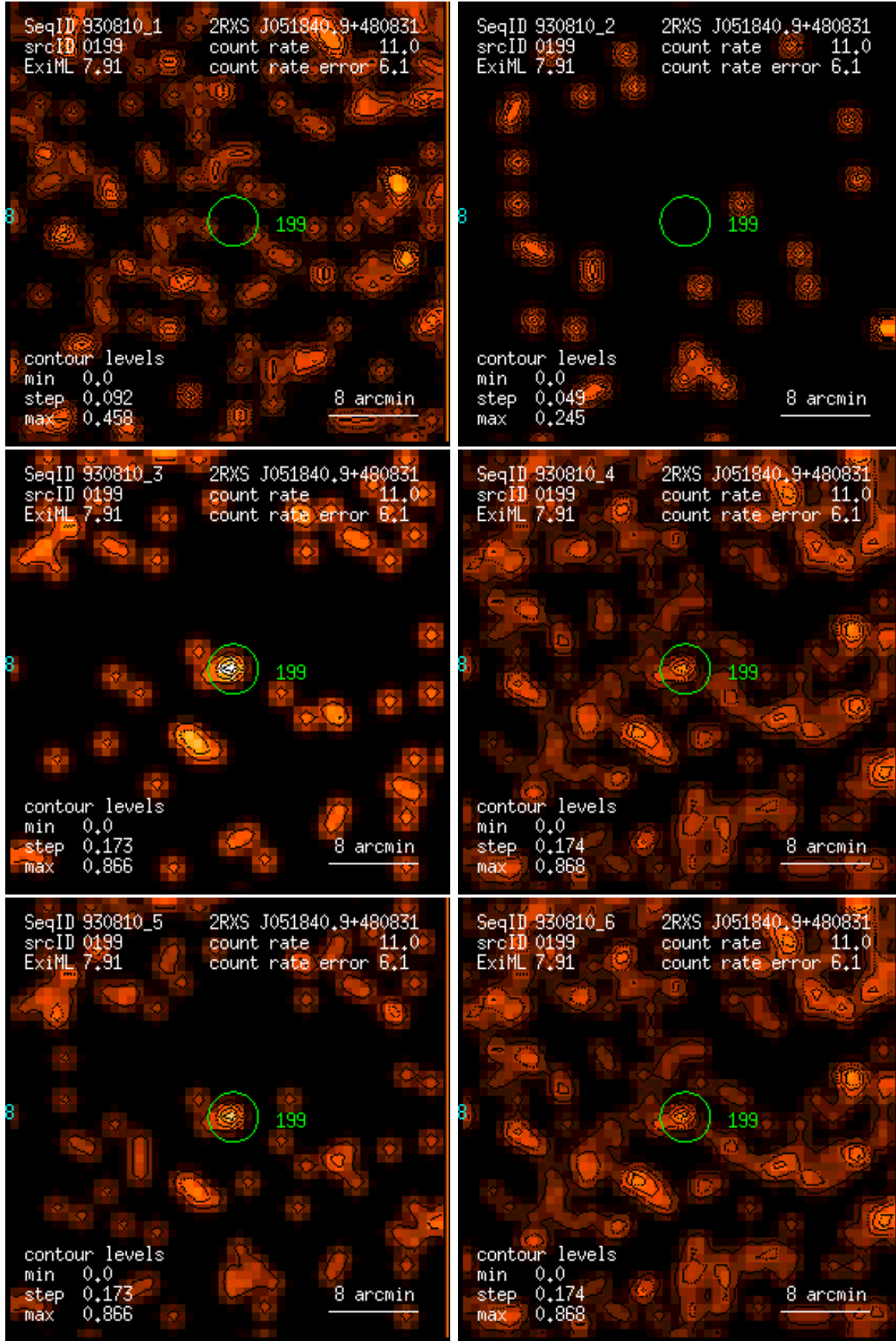
Figure 199: RASS 930810: detection 0199: band rate images, Gaussian filter: (1) PSPC channels 11 – 41, (2) 52 – 90, (3) 91 – 201, (4) 11 – 235, (5) 52 – 201, (6) 11 – 201. Broad band rates in counts/ks. Band rate contour levels in counts/ks/arcmin 2 .
