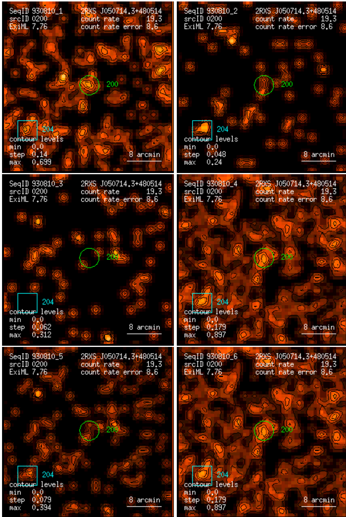
Figure 200: RASS 930810: detection 0200: band rate images, Gaussian filter: (1) PSPC channels 11 – 41, (2) 52 – 90, (3) 91 – 201, (4) 11 – 235, (5) 52 – 201, (6) 11 – 201. Broad band rates in counts/ks. Band rate contour levels in counts/ks/arcmin 2 .
