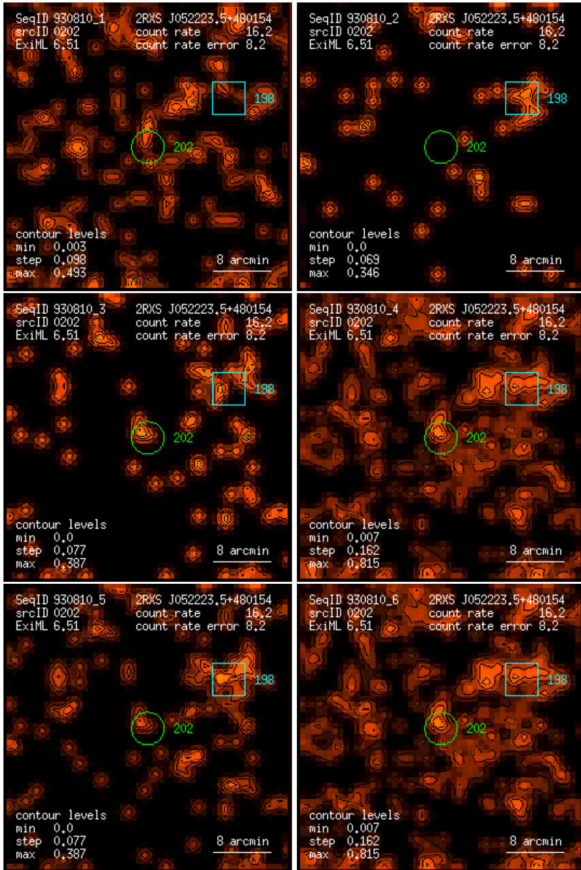
Figure 202: RASS 930810: detection 0202: band rate images, Gaussian filter: (1) PSPC channels 11 – 41, (2) 52 – 90, (3) 91 – 201, (4) 11 – 235, (5) 52 – 201, (6) 11 – 201. Broad band rates in counts/ks. Band rate contour levels in counts/ks/arcmin 2 .
