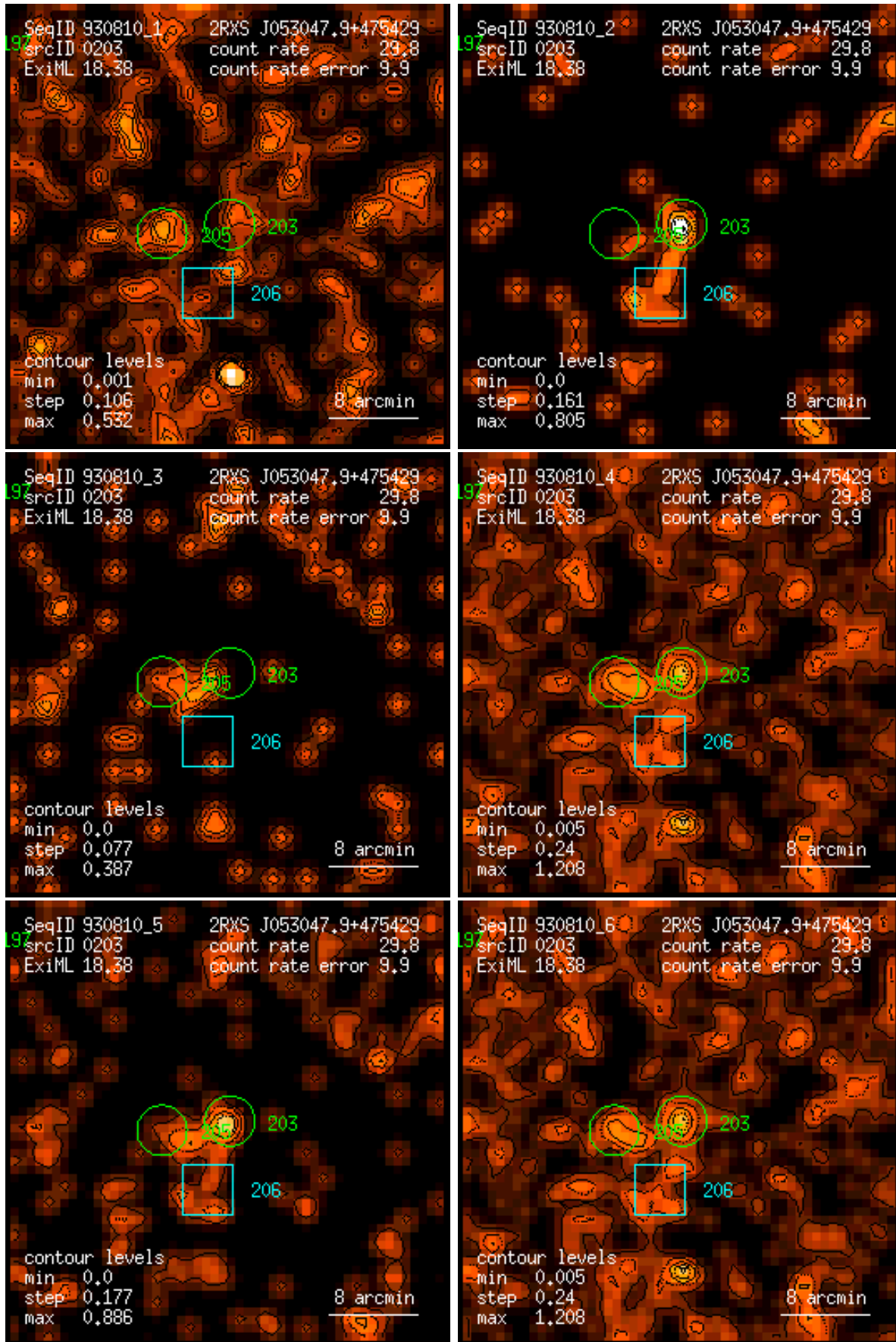
Figure 203: RASS 930810: detection 0203: band rate images, Gaussian filter: (1) PSPC channels 11 – 41, (2) 52 – 90, (3) 91 – 201, (4) 11 – 235, (5) 52 – 201, (6) 11 – 201. Broad band rates in counts/ks. Band rate contour levels in counts/ks/arcmin 2 .
