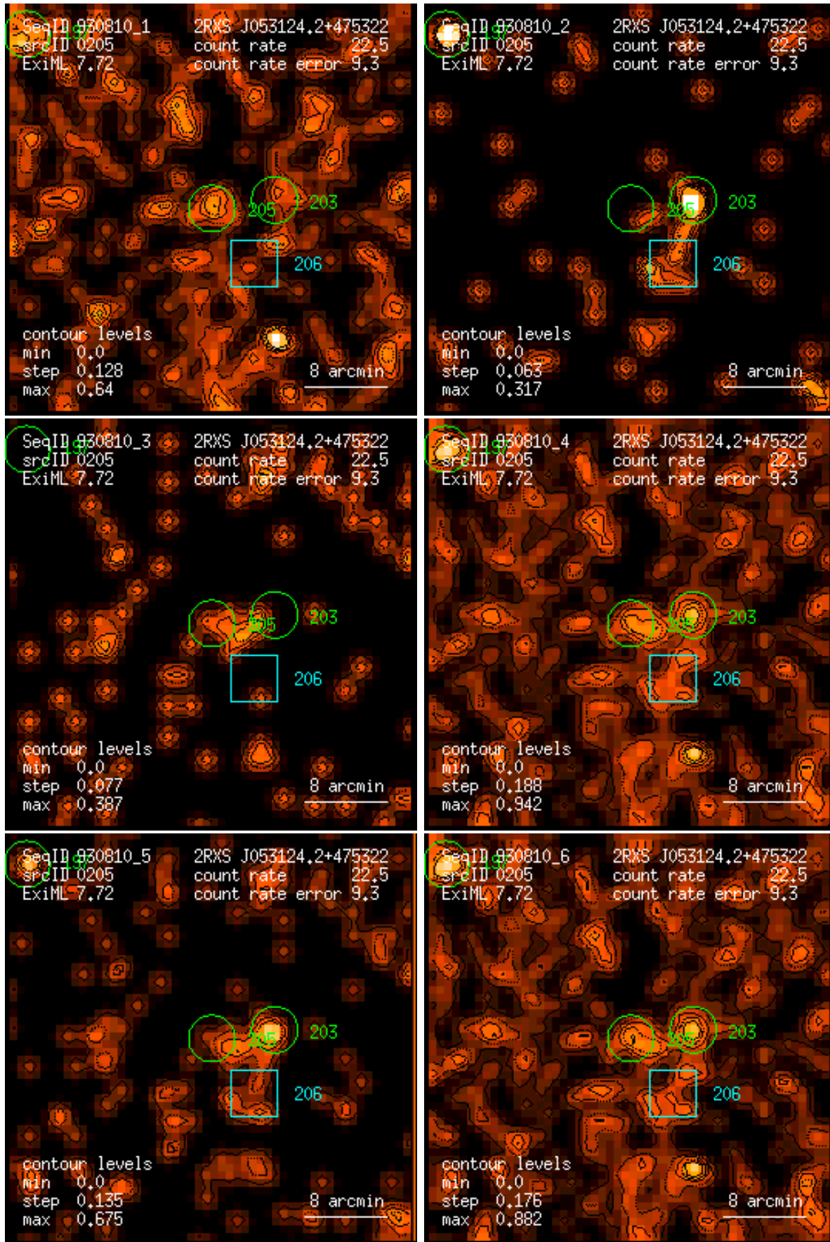
Figure 205: RASS 930810: detection 0205: band rate images, Gaussian filter: (1) PSPC channels 11 – 41, (2) 52 – 90, (3) 91 – 201, (4) 11 – 235, (5) 52 – 201, (6) 11 – 201. Broad band rates in counts/ks. Band rate contour levels in counts/ks/arcmin 2 .
