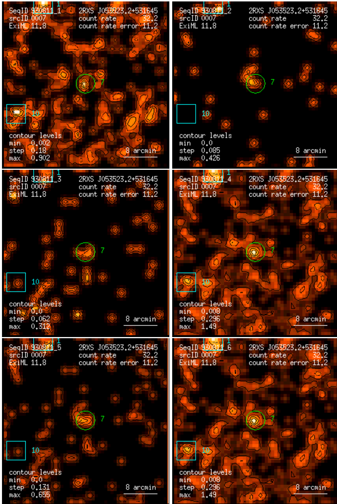
Figure 7: RASS 930811: detection 0007: band rate images, Gaussian filter: (1) PSPC channels 11 – 41, (2) 52 – 90, (3) 91 – 201, (4) 11 – 235, (5) 52 – 201, (6) 11 – 201. Broad band rates in counts/ks. Band rate contour levels in counts/ks/arcmin 2 .
