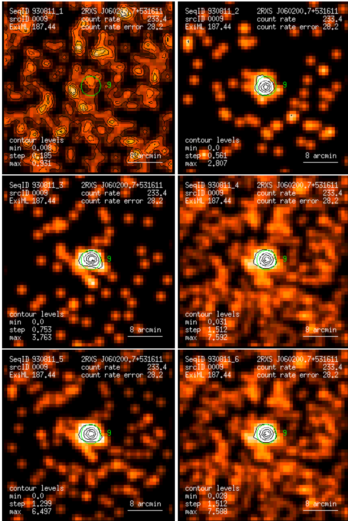
Figure 9: RASS 930811: detection 0009: band rate images, Gaussian filter: (1) PSPC channels 11 – 41, (2) 52 – 90, (3) 91 – 201, (4) 11 – 235, (5) 52 – 201, (6) 11 – 201. Broad band rates in counts/ks. Band rate contour levels in counts/ks/arcmin 2 .
