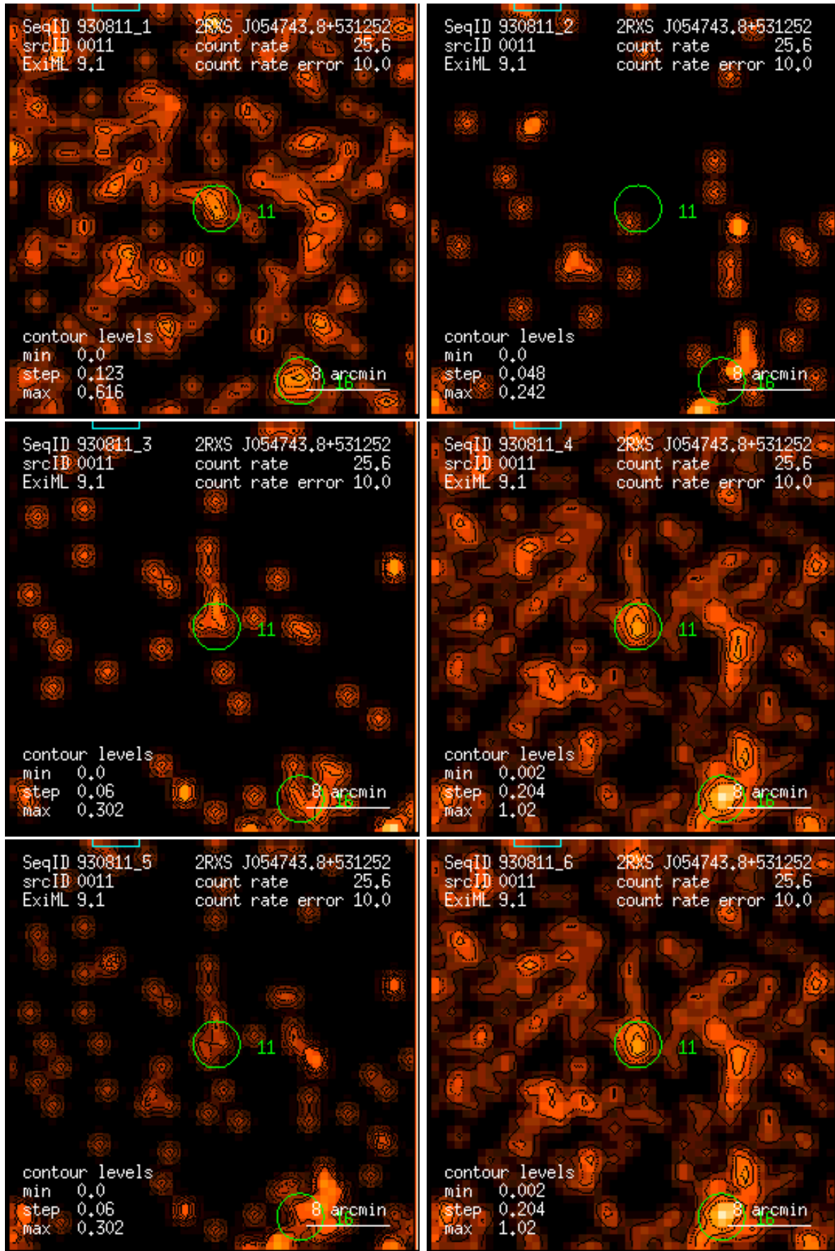
Figure 11: RASS 930811: detection 0011: band rate images, Gaussian filter: (1) PSPC channels 11 – 41, (2) 52 – 90, (3) 91 – 201, (4) 11 – 235, (5) 52 – 201, (6) 11 – 201. Broad band rates in counts/ks. Band rate contour levels in counts/ks/arcmin 2 .
