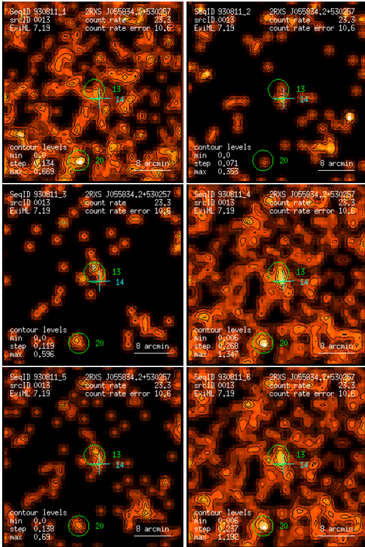
Figure 13: RASS 930811: detection 0013: band rate images, Gaussian filter: (1) PSPC channels 11 – 41, (2) 52 – 90, (3) 91 – 201, (4) 11 – 235, (5) 52 – 201, (6) 11 – 201. Broad band rates in counts/ks. Band rate contour levels in counts/ks/arcmin 2 .
