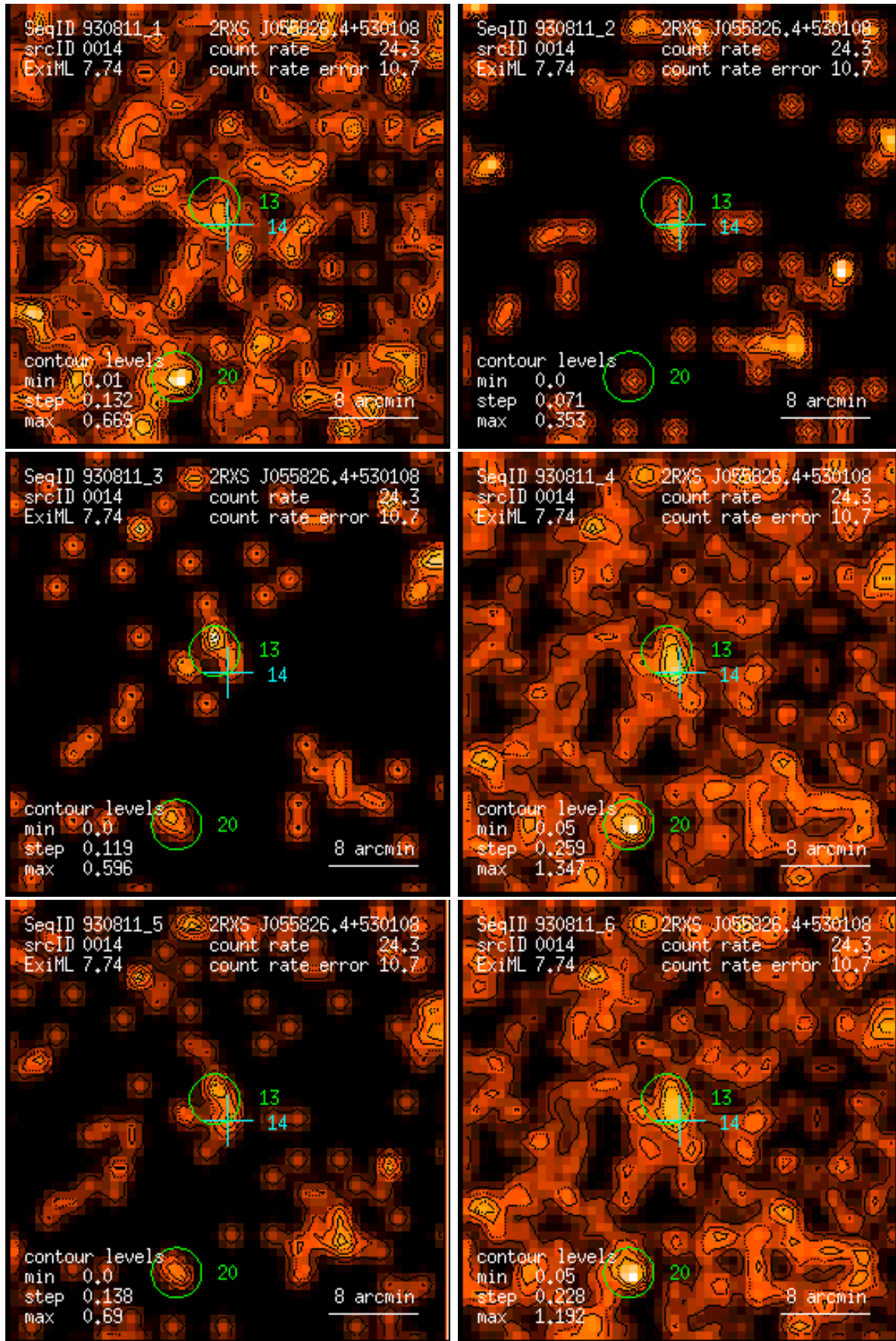
Figure 14: RASS 930811: detection 0014: band rate images, Gaussian filter: (1) PSPC channels 11 – 41, (2) 52 – 90, (3) 91 – 201, (4) 11 – 235, (5) 52 – 201, (6) 11 – 201. Broad band rates in counts/ks. Band rate contour levels in counts/ks/arcmin 2 .
