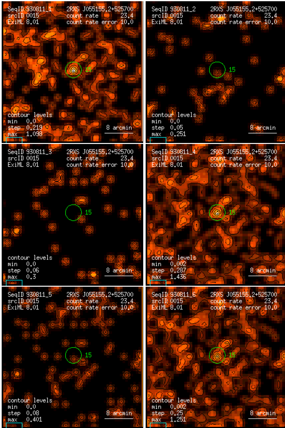
Figure 15: RASS 930811: detection 0015: band rate images, Gaussian filter: (1) PSPC channels 11 – 41, (2) 52 – 90, (3) 91 – 201, (4) 11 – 235, (5) 52 – 201, (6) 11 – 201. Broad band rates in counts/ks. Band rate contour levels in counts/ks/arcmin 2 .
