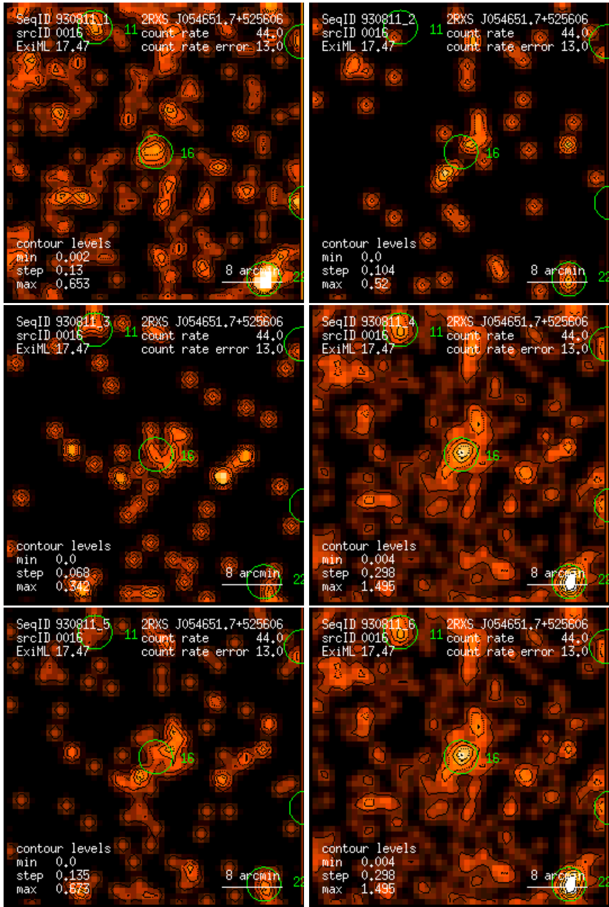
Figure 16: RASS 930811: detection 0016: band rate images, Gaussian filter: (1) PSPC channels 11 – 41, (2) 52 – 90, (3) 91 – 201, (4) 11 – 235, (5) 52 – 201, (6) 11 – 201. Broad band rates in counts/ks. Band rate contour levels in counts/ks/arcmin 2 .
