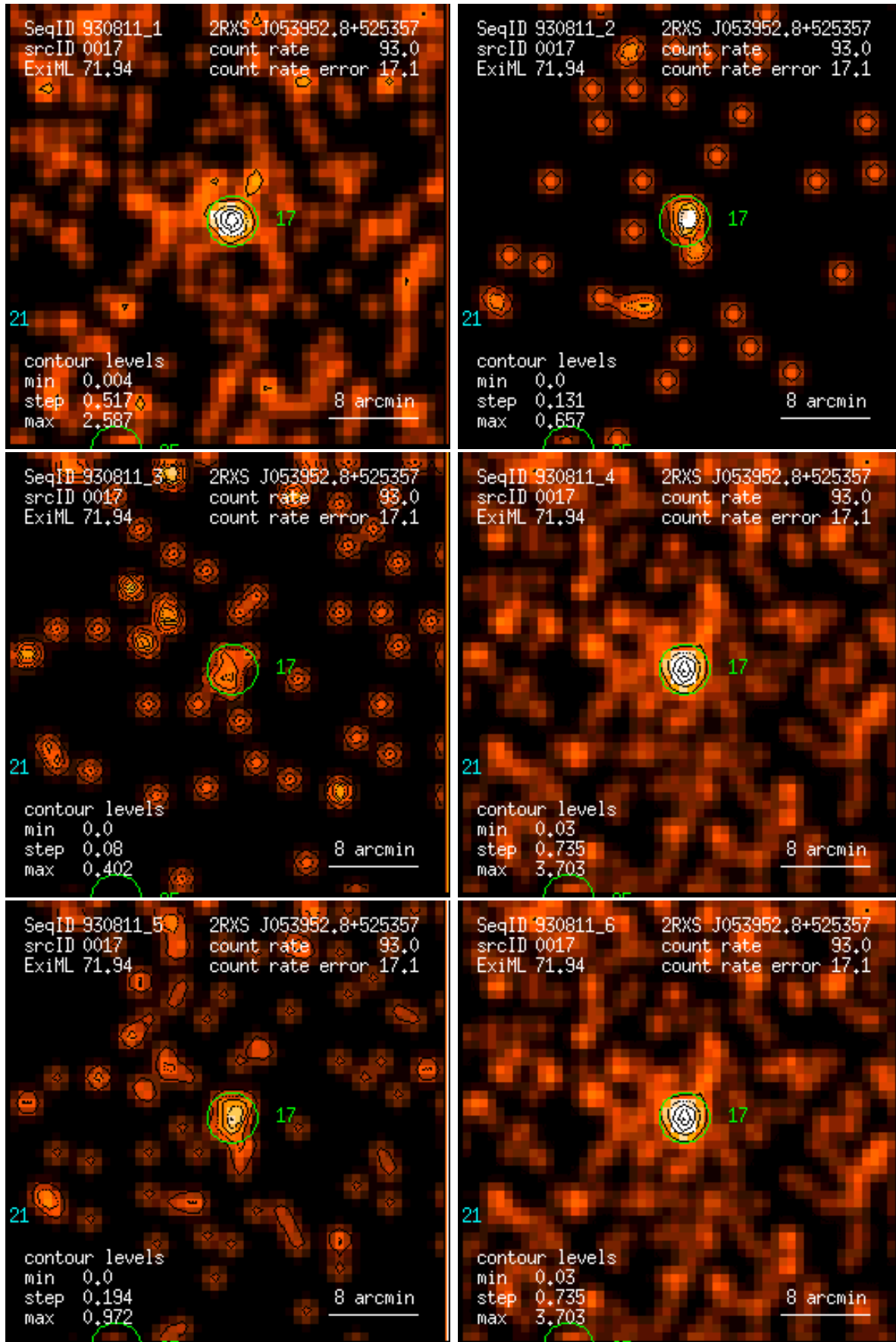
Figure 17: RASS 930811: detection 0017: band rate images, Gaussian filter: (1) PSPC channels 11 – 41, (2) 52 – 90, (3) 91 – 201, (4) 11 – 235, (5) 52 – 201, (6) 11 – 201. Broad band rates in counts/ks. Band rate contour levels in counts/ks/arcmin 2 .
