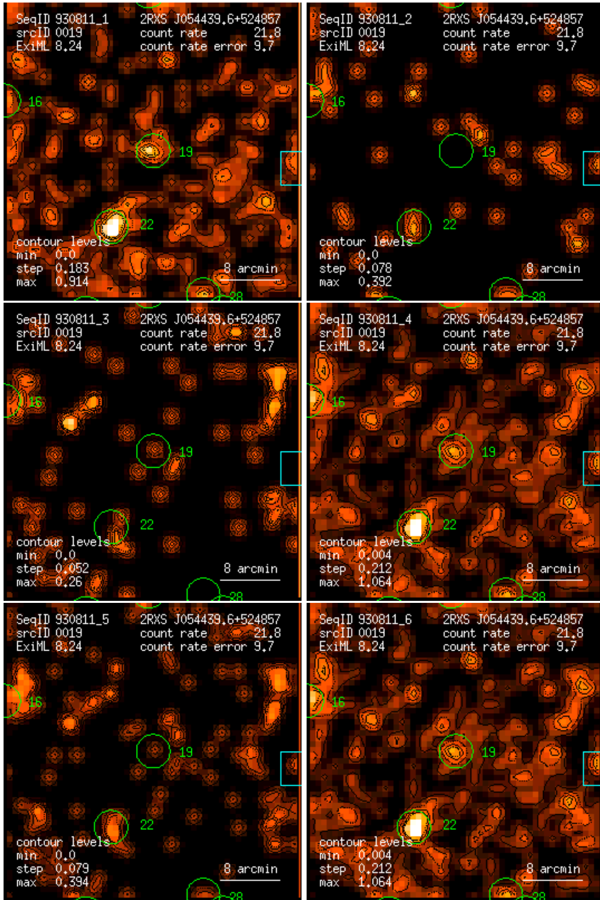
Figure 19: RASS 930811: detection 0019: band rate images, Gaussian filter: (1) PSPC channels 11 – 41, (2) 52 – 90, (3) 91 – 201, (4) 11 – 235, (5) 52 – 201, (6) 11 – 201. Broad band rates in counts/ks. Band rate contour levels in counts/ks/arcmin 2 .
