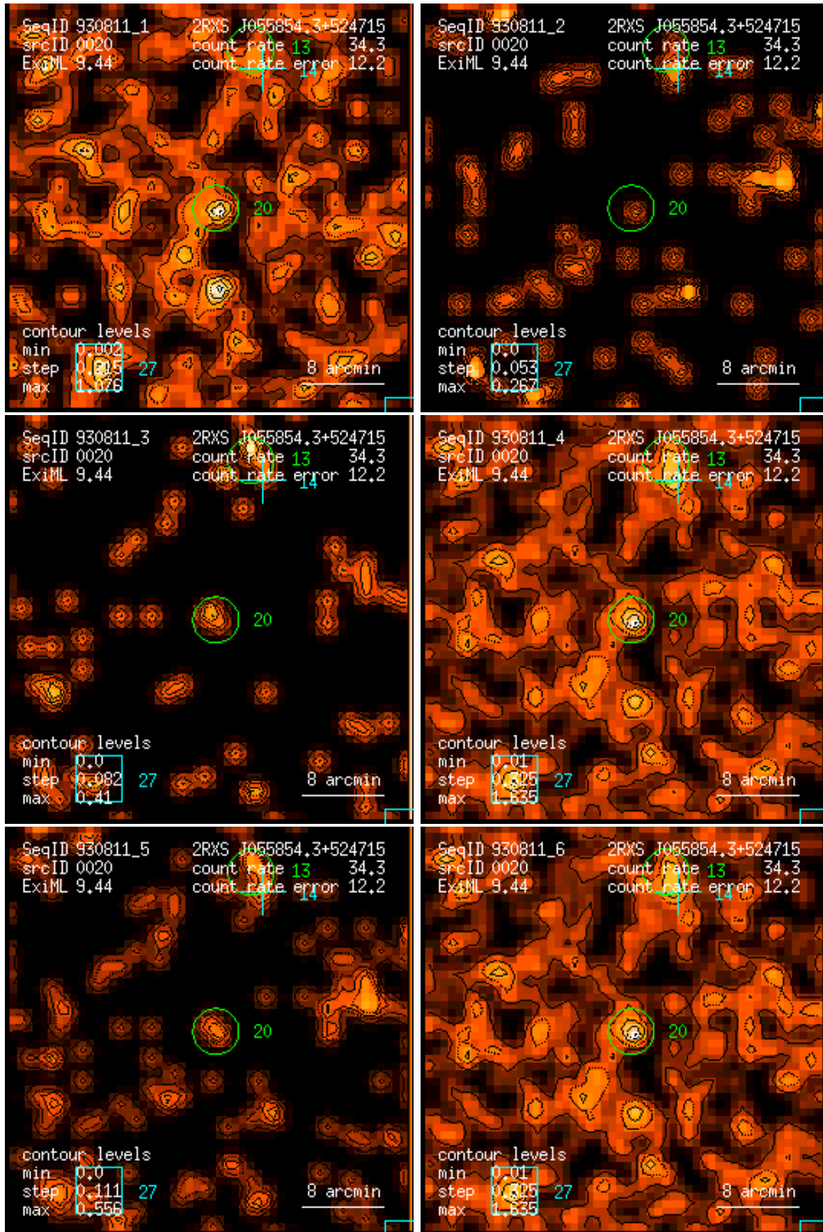
Figure 20: RASS 930811: detection 0020: band rate images, Gaussian filter: (1) PSPC channels 11 – 41, (2) 52 – 90, (3) 91 – 201, (4) 11 – 235, (5) 52 – 201, (6) 11 – 201. Broad band rates in counts/ks. Band rate contour levels in counts/ks/arcmin 2 .
