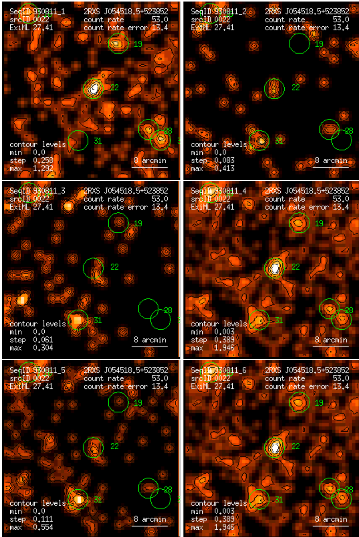
Figure 22: RASS 930811: detection 0022: band rate images, Gaussian filter: (1) PSPC channels 11 – 41, (2) 52 – 90, (3) 91 – 201, (4) 11 – 235, (5) 52 – 201, (6) 11 – 201. Broad band rates in counts/ks. Band rate contour levels in counts/ks/arcmin 2 .
