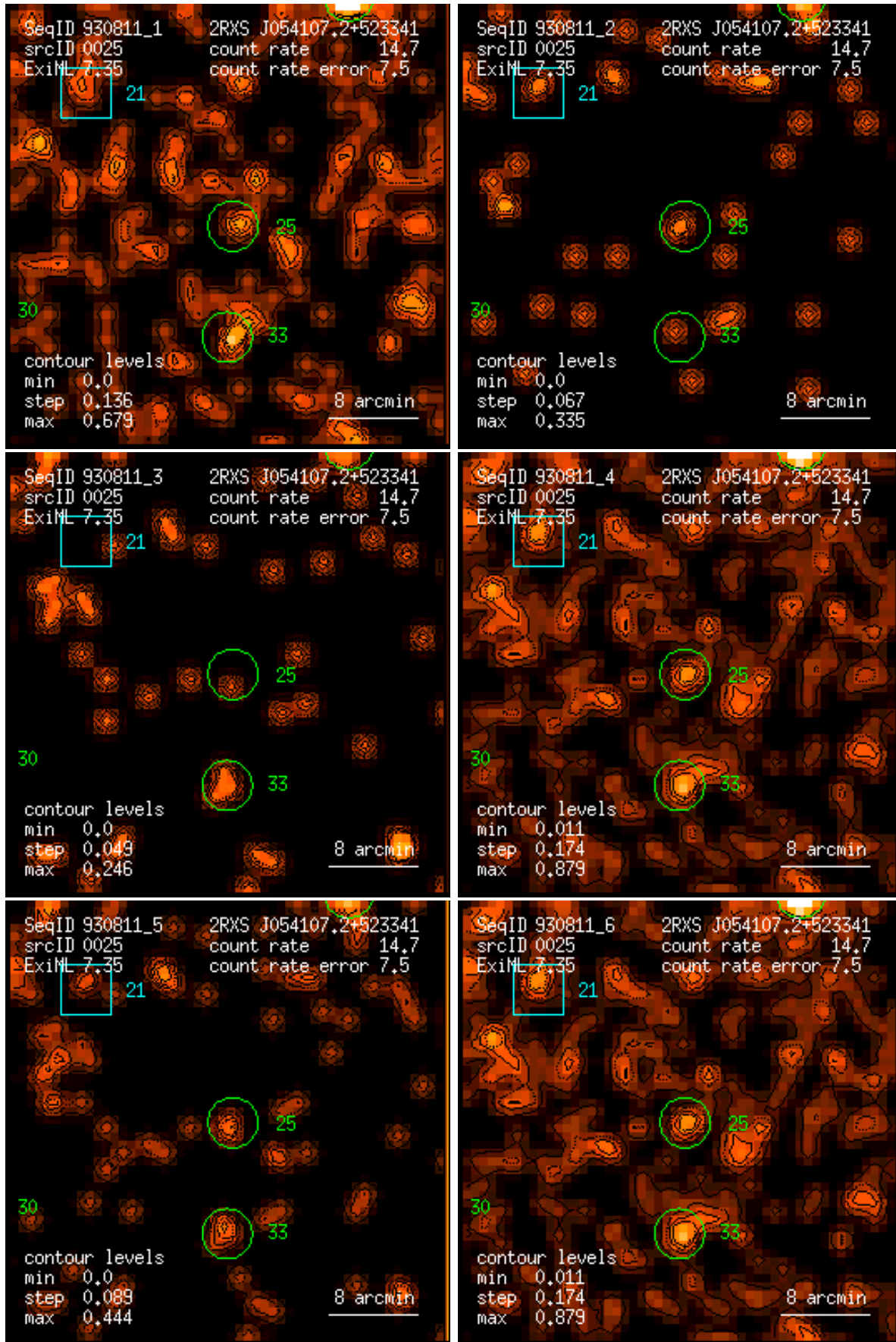
Figure 25: RASS 930811: detection 0025: band rate images, Gaussian filter: (1) PSPC channels 11 – 41, (2) 52 – 90, (3) 91 – 201, (4) 11 – 235, (5) 52 – 201, (6) 11 – 201. Broad band rates in counts/ks. Band rate contour levels in counts/ks/arcmin 2 .
