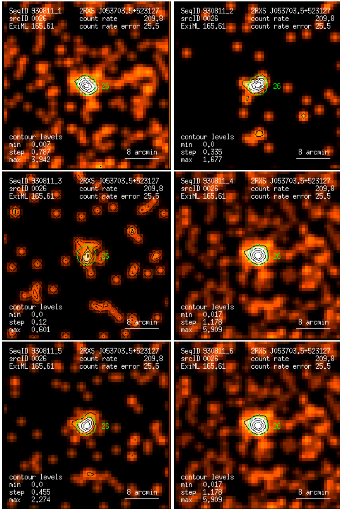
Figure 26: RASS 930811: detection 0026: band rate images, Gaussian filter: (1) PSPC channels 11 – 41, (2) 52 – 90, (3) 91 – 201, (4) 11 – 235, (5) 52 – 201, (6) 11 – 201. Broad band rates in counts/ks. Band rate contour levels in counts/ks/arcmin 2 .
