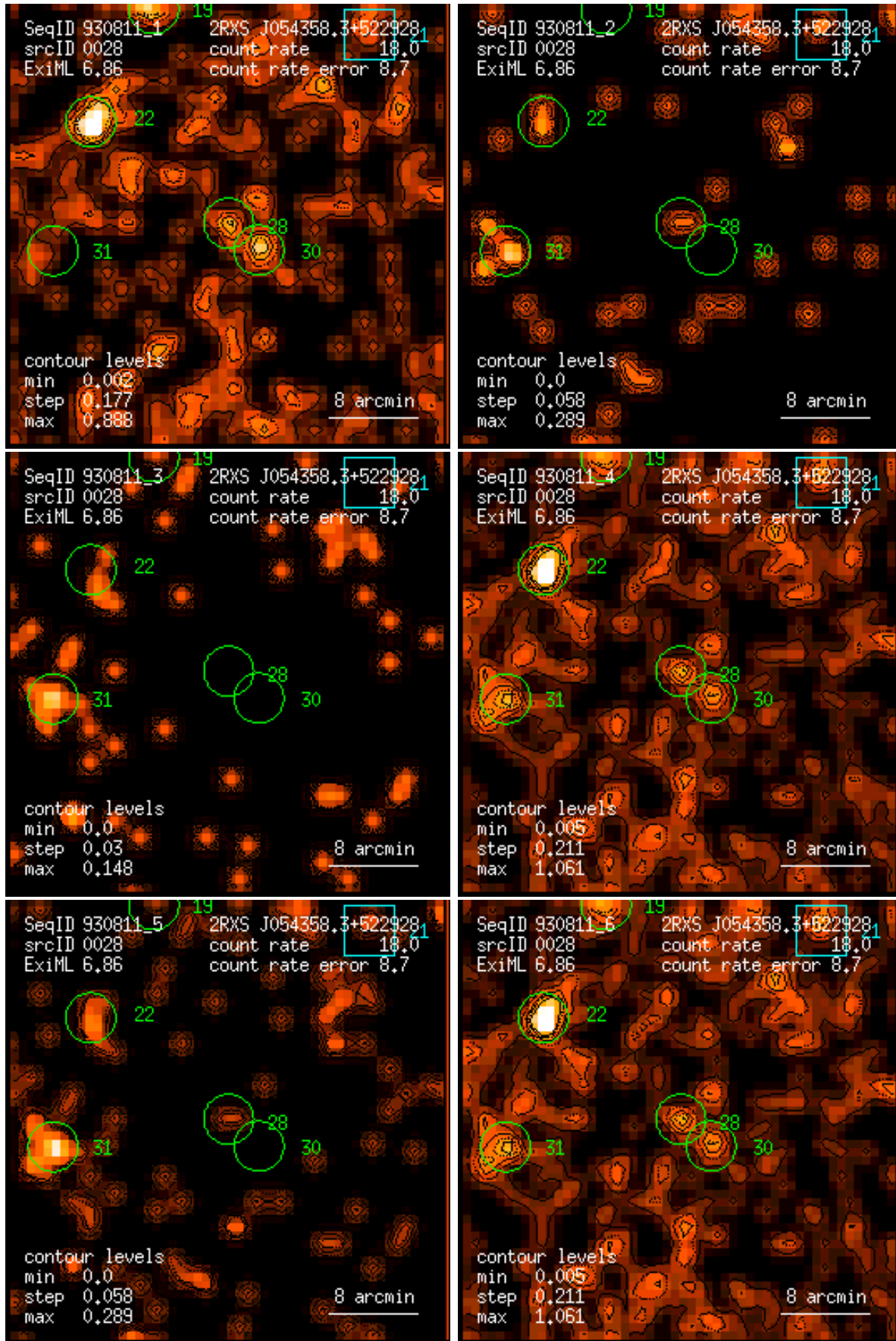
Figure 28: RASS 930811: detection 0028: band rate images, Gaussian filter: (1) PSPC channels 11 – 41, (2) 52 – 90, (3) 91 – 201, (4) 11 – 235, (5) 52 – 201, (6) 11 – 201. Broad band rates in counts/ks. Band rate contour levels in counts/ks/arcmin 2 .
