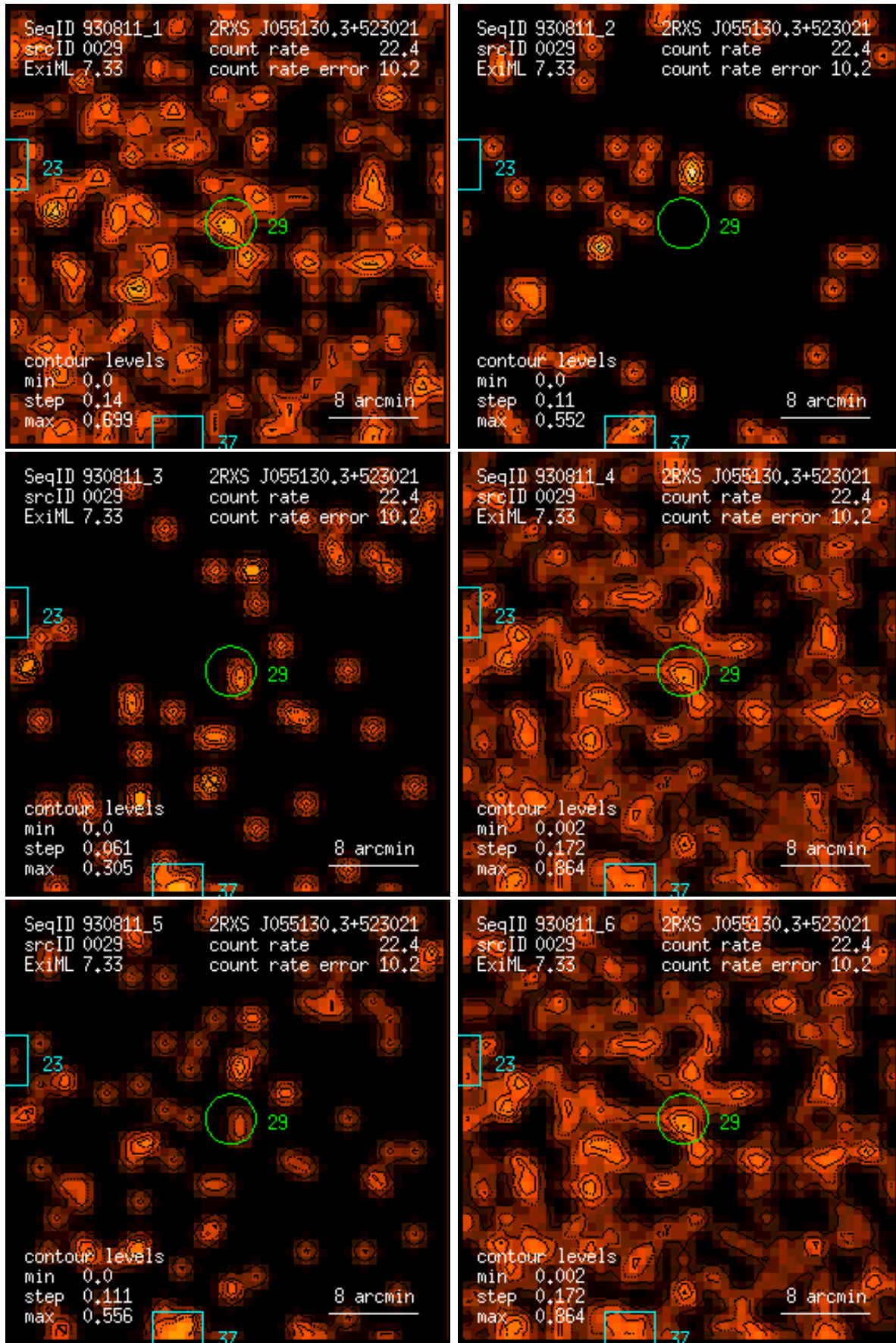
Figure 29: RASS 930811: detection 0029: band rate images, Gaussian filter: (1) PSPC channels 11 – 41, (2) 52 – 90, (3) 91 – 201, (4) 11 – 235, (5) 52 – 201, (6) 11 – 201. Broad band rates in counts/ks. Band rate contour levels in counts/ks/arcmin 2 .
