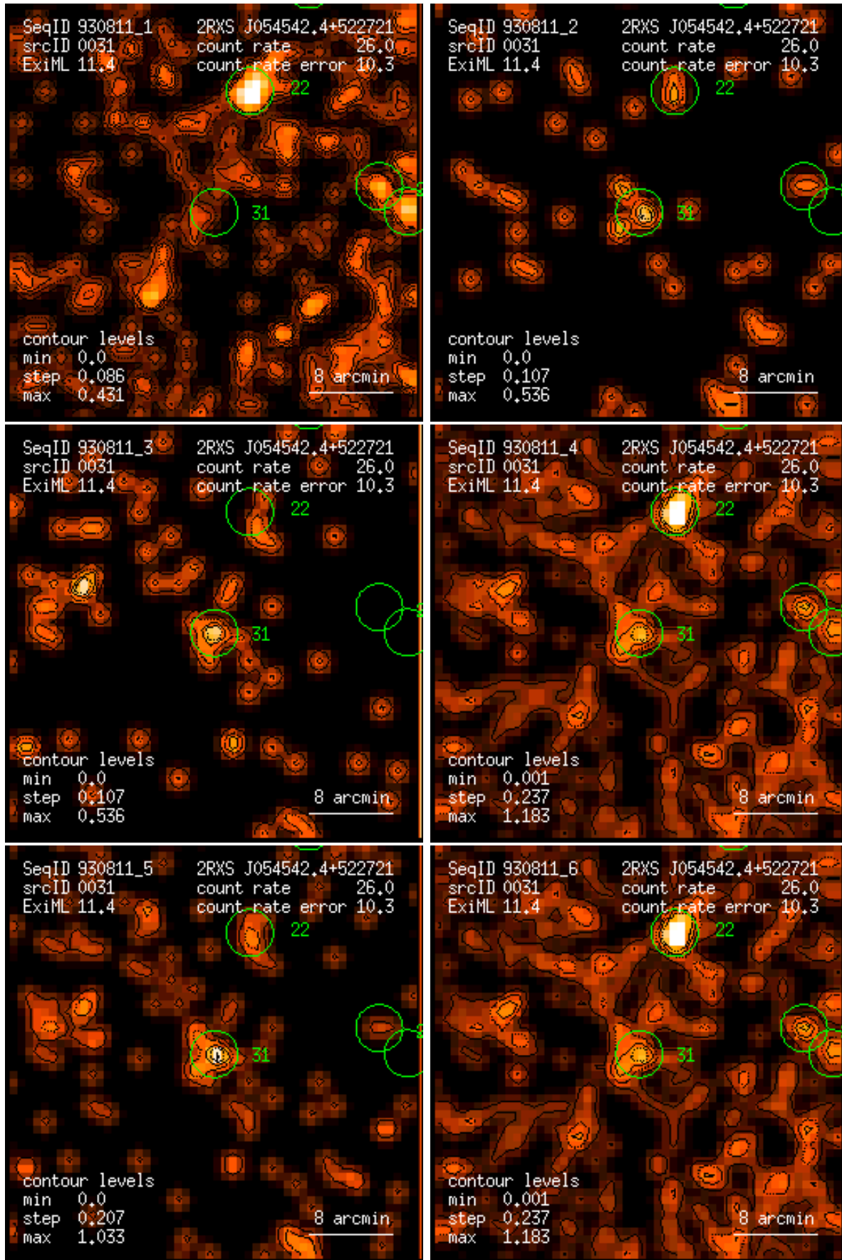
Figure 31: RASS 930811: detection 0031: band rate images, Gaussian filter: (1) PSPC channels 11 – 41, (2) 52 – 90, (3) 91 – 201, (4) 11 – 235, (5) 52 – 201, (6) 11 – 201. Broad band rates in counts/ks. Band rate contour levels in counts/ks/arcmin 2 .
