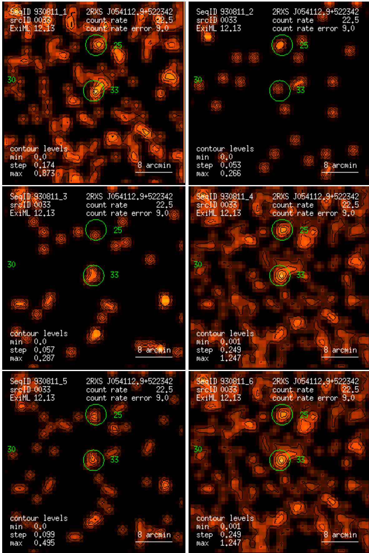
Figure 33: RASS 930811: detection 0033: band rate images, Gaussian filter: (1) PSPC channels 11 – 41, (2) 52 – 90, (3) 91 – 201, (4) 11 – 235, (5) 52 – 201, (6) 11 – 201. Broad band rates in counts/ks. Band rate contour levels in counts/ks/arcmin 2 .
