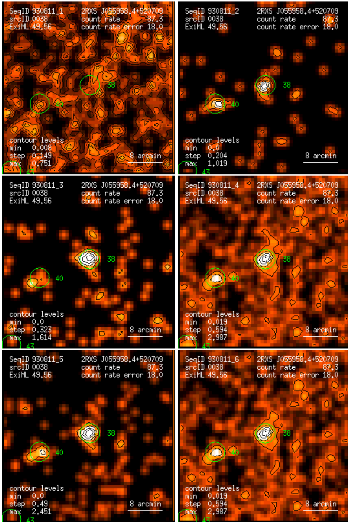
Figure 38: RASS 930811: detection 0038: band rate images, Gaussian filter: (1) PSPC channels 11 – 41, (2) 52 – 90, (3) 91 – 201, (4) 11 – 235, (5) 52 – 201, (6) 11 – 201. Broad band rates in counts/ks. Band rate contour levels in counts/ks/arcmin 2 .
