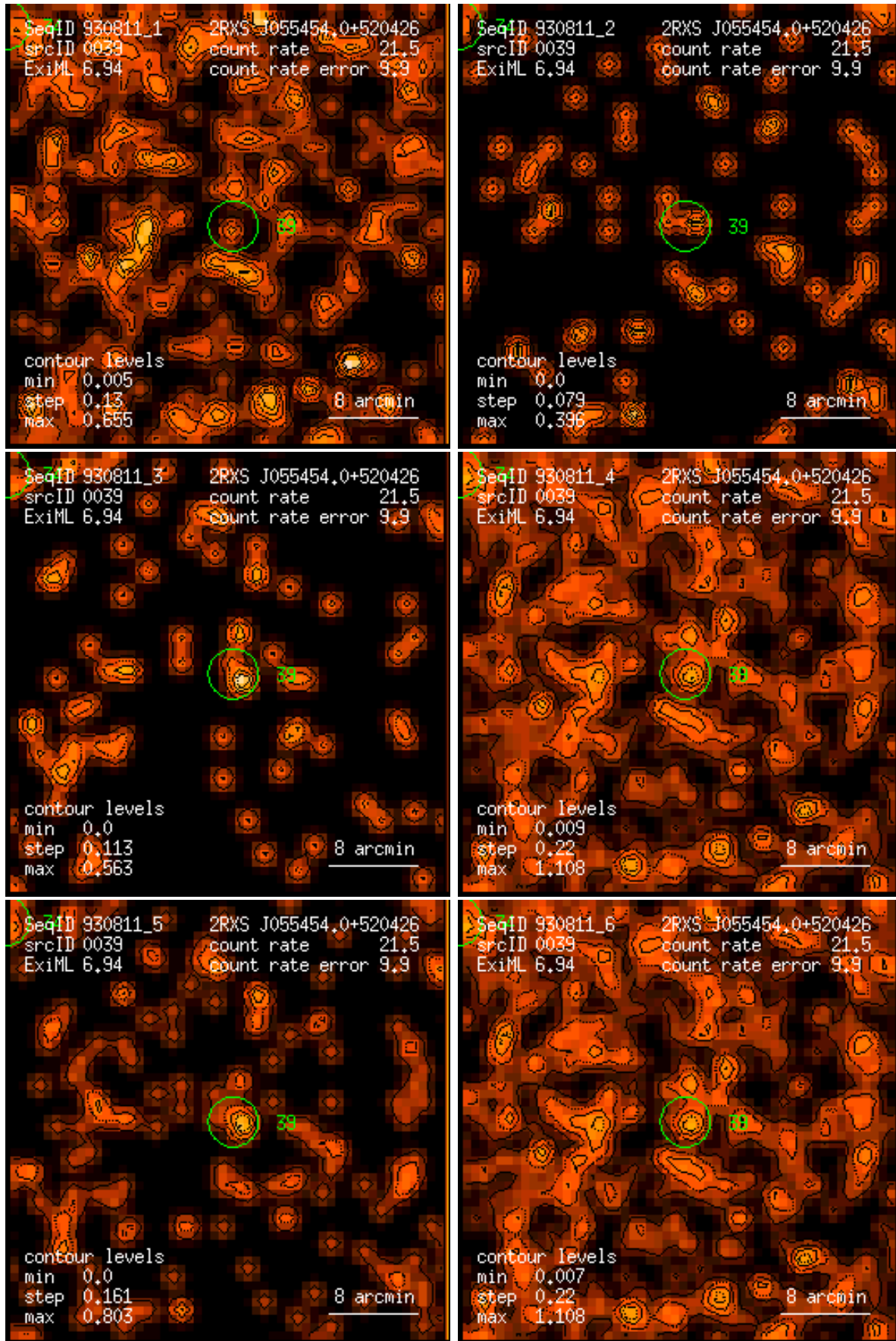
Figure 39: RASS 930811: detection 0039: band rate images, Gaussian filter: (1) PSPC channels 11 – 41, (2) 52 – 90, (3) 91 – 201, (4) 11 – 235, (5) 52 – 201, (6) 11 – 201. Broad band rates in counts/ks. Band rate contour levels in counts/ks/arcmin 2 .
