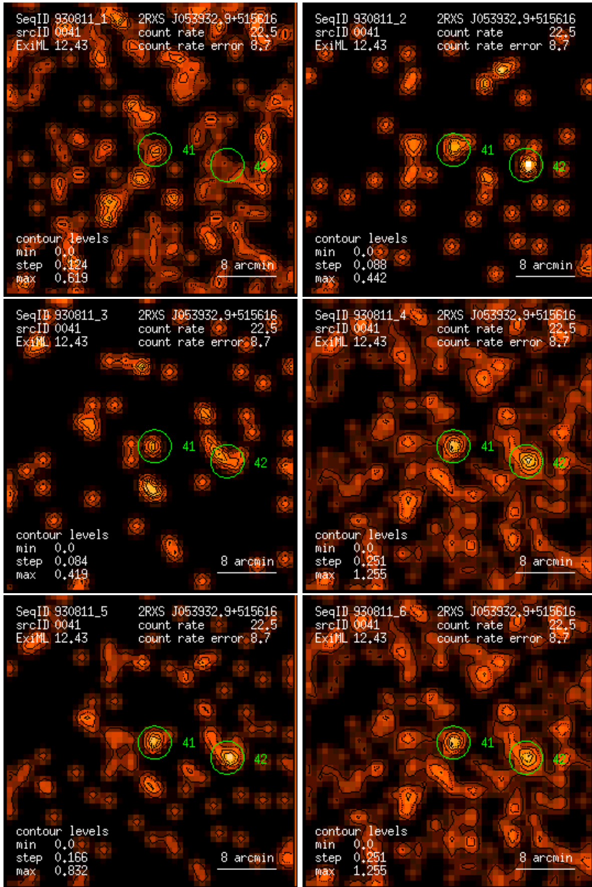
Figure 41: RASS 930811: detection 0041: band rate images, Gaussian filter: (1) PSPC channels 11 – 41, (2) 52 – 90, (3) 91 – 201, (4) 11 – 235, (5) 52 – 201, (6) 11 – 201. Broad band rates in counts/ks. Band rate contour levels in counts/ks/arcmin 2 .
