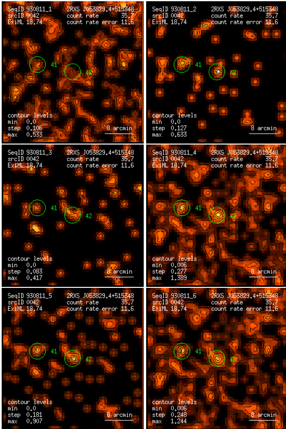
Figure 42: RASS 930811: detection 0042: band rate images, Gaussian filter: (1) PSPC channels 11 – 41, (2) 52 – 90, (3) 91 – 201, (4) 11 – 235, (5) 52 – 201, (6) 11 – 201. Broad band rates in counts/ks. Band rate contour levels in counts/ks/arcmin 2 .
